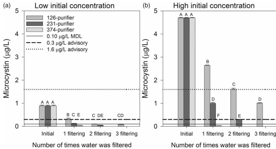
Figure 2 | Total microcystins concentration in the two repeated filtering experiments, (a) with low initial concentration and (b) with high initial concentration. Water was percolated through the 126-purifiers three times, the 231-purifiers twice, and the 374-purifiers just once. Bars are means ( \pm 1 standard error) of three replicate pitchers. Letters above bars and horizontal lines follow the Figure 1 caption.
