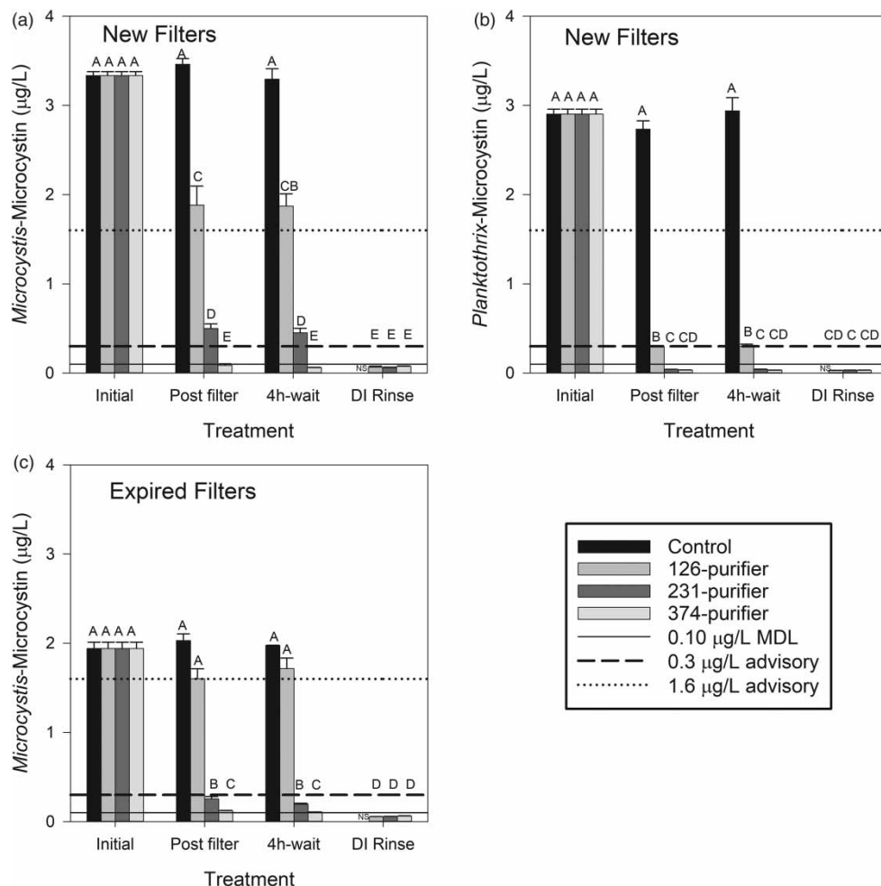
Figure 1 | Total microcystin concentration ( \mu\text{g/L} ) following percolation through pitcher-style purifiers ('post filter'), 4 hours after percolation ('4h-wait'), and in deionized water percolated ('DI rinse'). Experiments were conducted with new filter cartridges with microcystins extracted from (a) Microcystis and (b) Planktothrix and (c) with expired cartridges using Microcystis -microcystins. Bars are means ( \pm 1 standard error) of three replicate pitchers. Letters above bars are Tukey test results with mean of A > B > C > D > E . Horizontal lines indicate the method detection limit, advisory level for children, and the advisory level for adults. 'NS' = no sample. DI water was not poured into the non-filtered controls.
