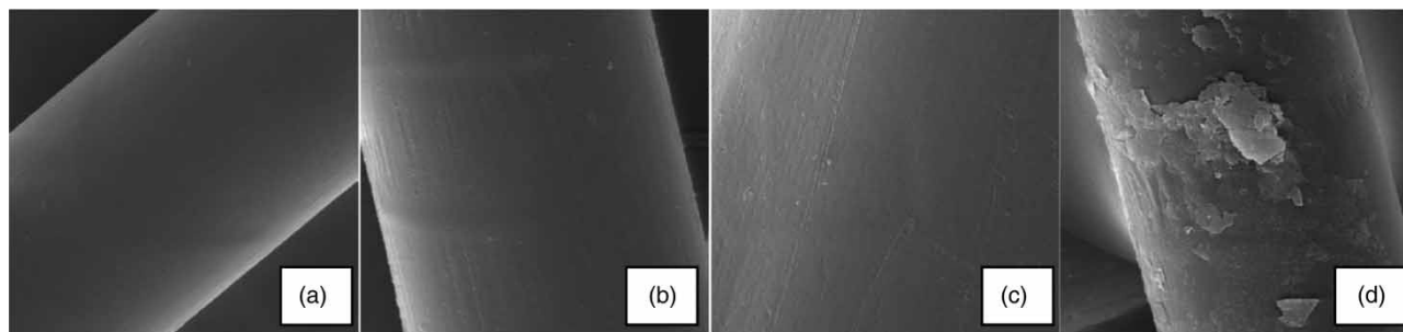
Figure 2 | Images from scanning electron microscopy with magnification of 2,000 \times : (a) without any treatment or use as filter media, (b) after solubility assay in hydrochloric acid, (c) after solubility assay in sodium hydroxide, (d) after use as filtering material for 3 months.
