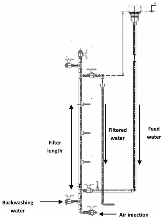
Figure 1 | Scheme of the fiber filter used in this study.
