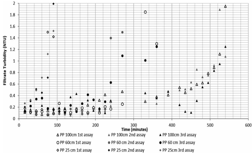
Figure 3 | Filtrate turbidity evolution for filters studied and for the application rate of 20 m/h.
