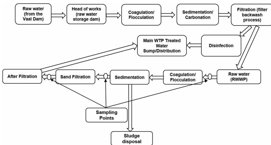
Figure 1 | Schematic of the RWWP showing the sequence of purification processes (coagulation, flocculation, sedimentation and sand filtration) and included sampling points, linked to the main water treatment plant.
