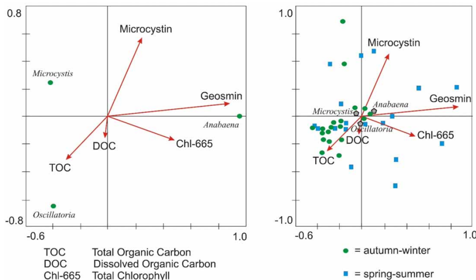
Figure 2 | CCA multivariate statistical results for cyanobacteria genera and associated organic compounds.
