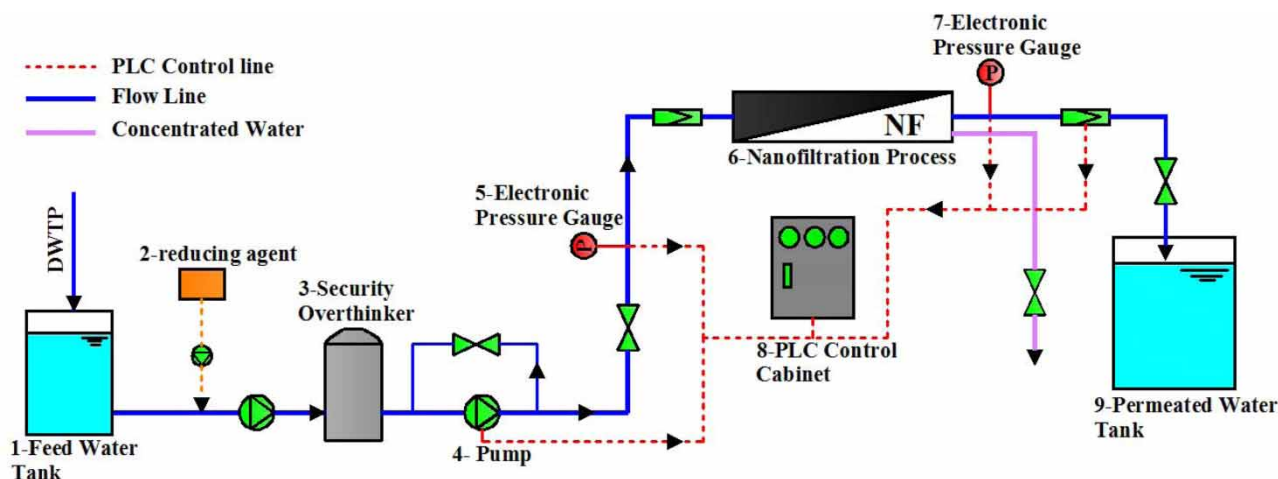
Figure 1 | A schematic diagram of the pilot-plant system.
