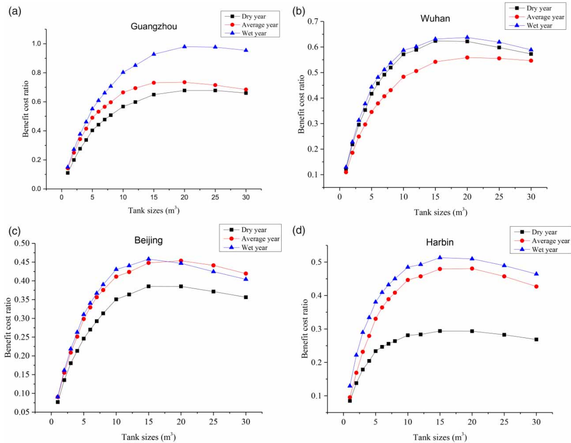
Figure 5 | Effects of tank sizes on the benefit–cost ratio of the proposed RWH system across four locations: (a) Guangzhou, (b) Wuhan, (c) Beijing and (d) Harbin.
