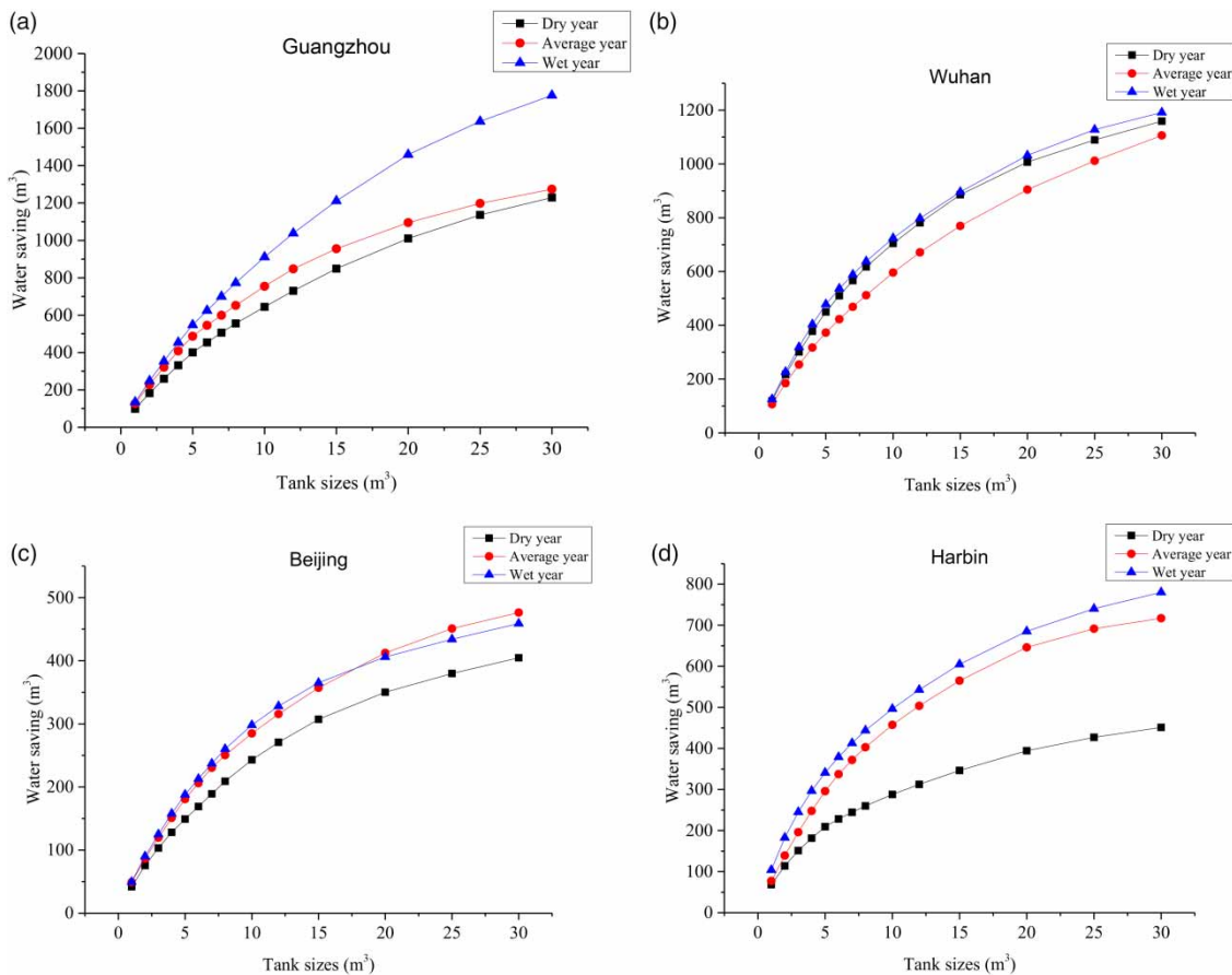
Figure 4 | Annual water saving in four cities: (a) Guangzhou, (b) Wuhan, (c) Beijing and (d) Harbin.
