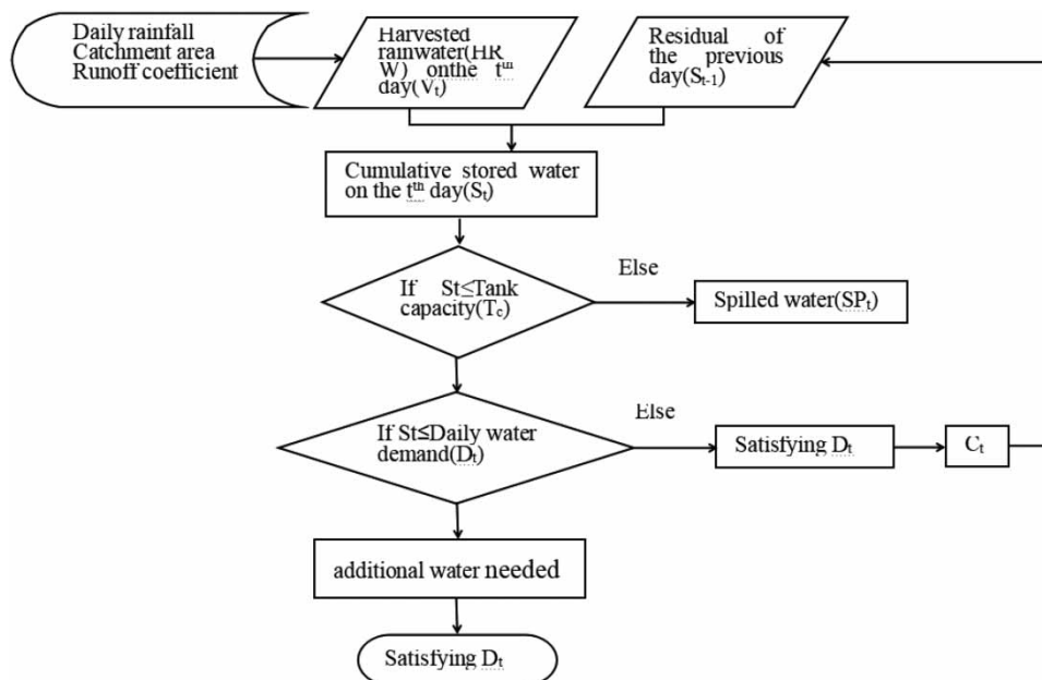
Figure 2 | Flowchart of daily water balance model.
