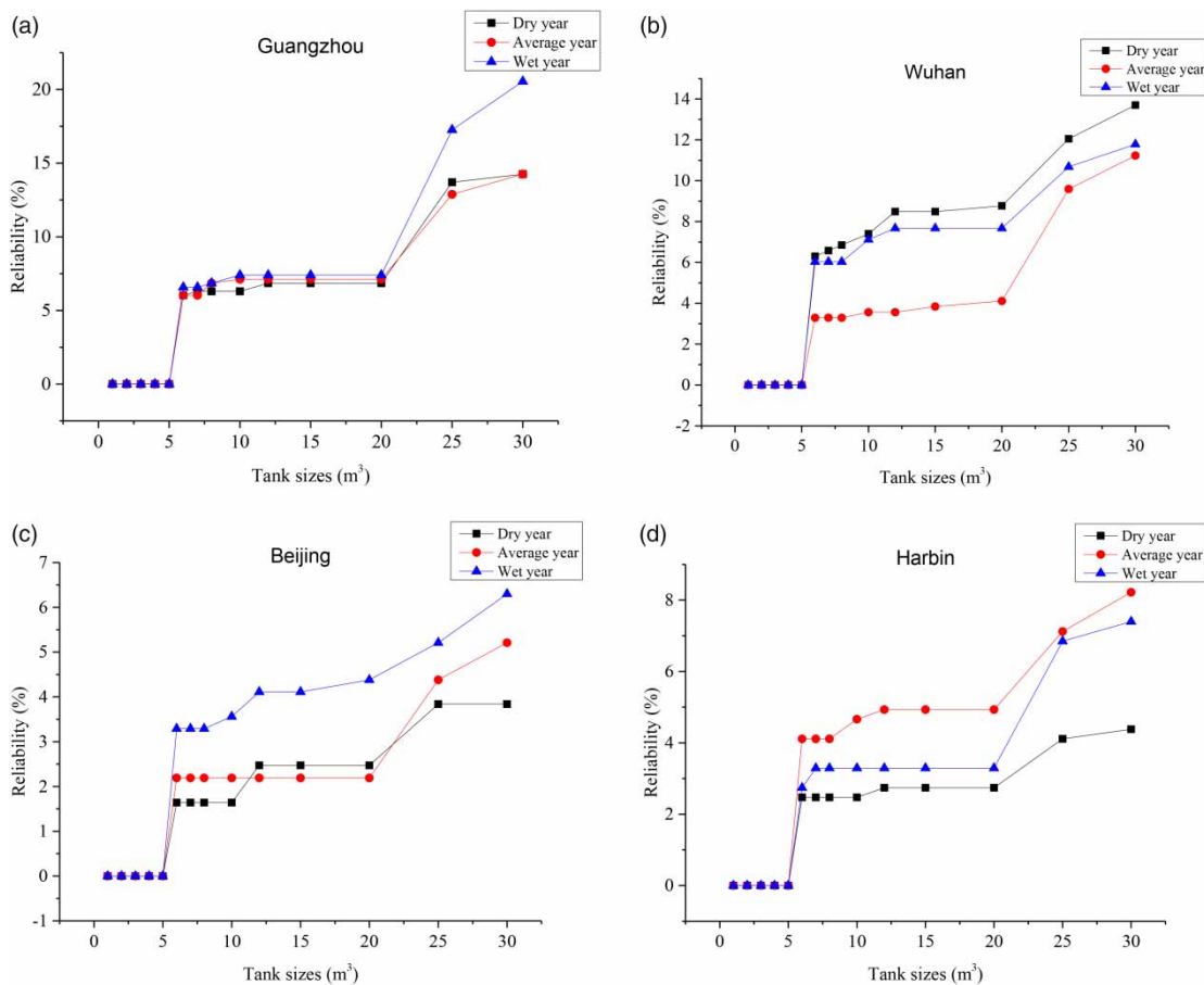
Figure 3 | Effects of tank sizes on the reliability of the proposed RWH system across four locations: (a) Guangzhou, (b) Wuhan, (c) Beijing and (d) Harbin.
