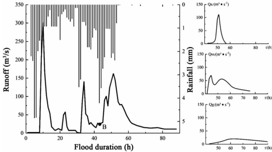
Figure 2 | The schematic diagram of runoff generation discrimination.
