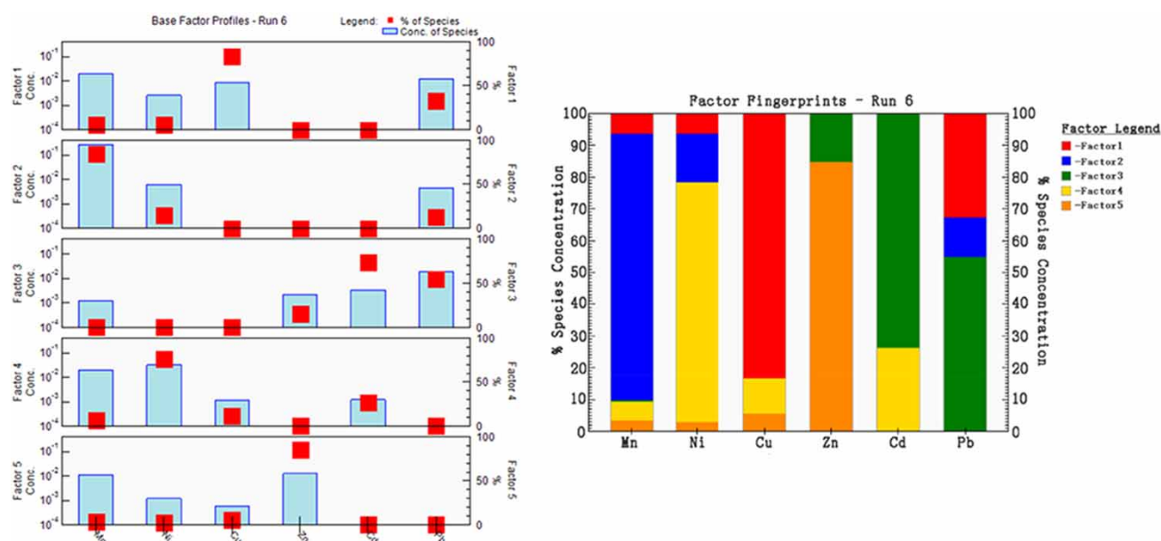
Figure 3 | Factor distribution and source contribution of PTEs in the PMF model.
