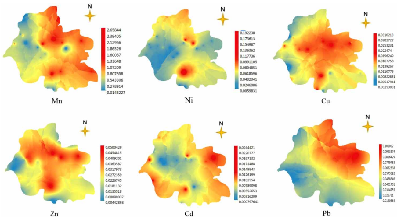
Figure 2 | Spatial distribution of each PTE (mg/L).
