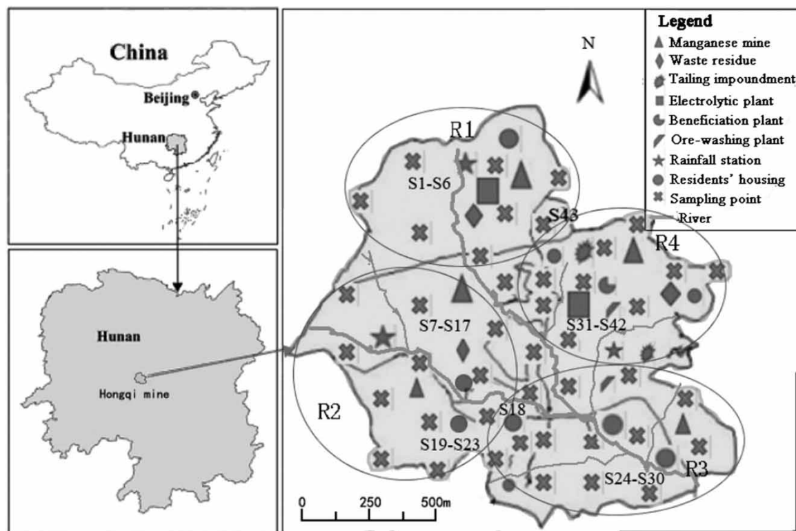
Figure 1 | Sampling location map.
