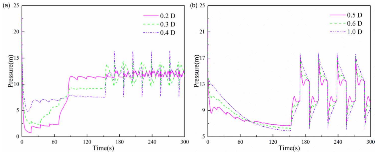
Figure 6 | Process line of pressure change at the bottom of one-way surge tank.
