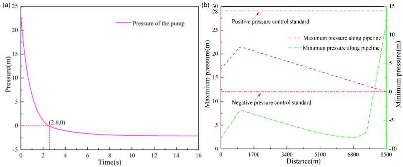
Figure 5 | (a) Pressure change after the pump is powered off; (b) pipeline pressure envelope without protection.
