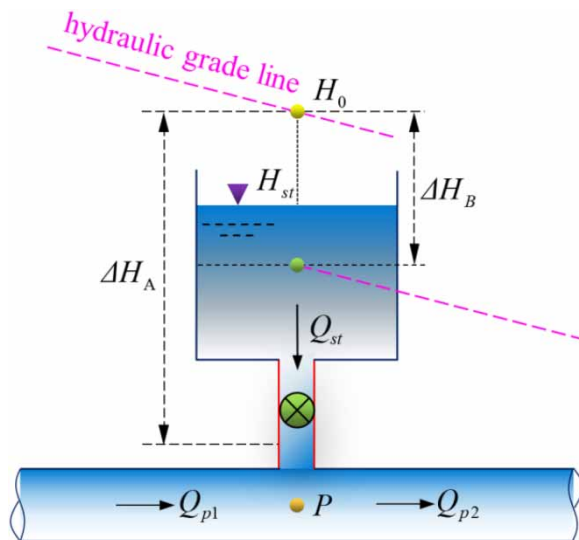
Figure 2 | Schematic of the pressure drop process of one-way surge tank.
