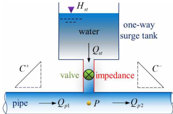
Figure 1 | Schematic of impedance one-way surge tank.
