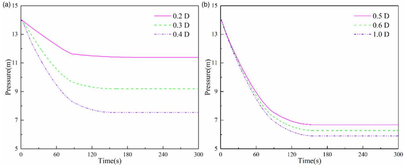
Figure 7 | Process line of water-level change of one-way surge tank.
