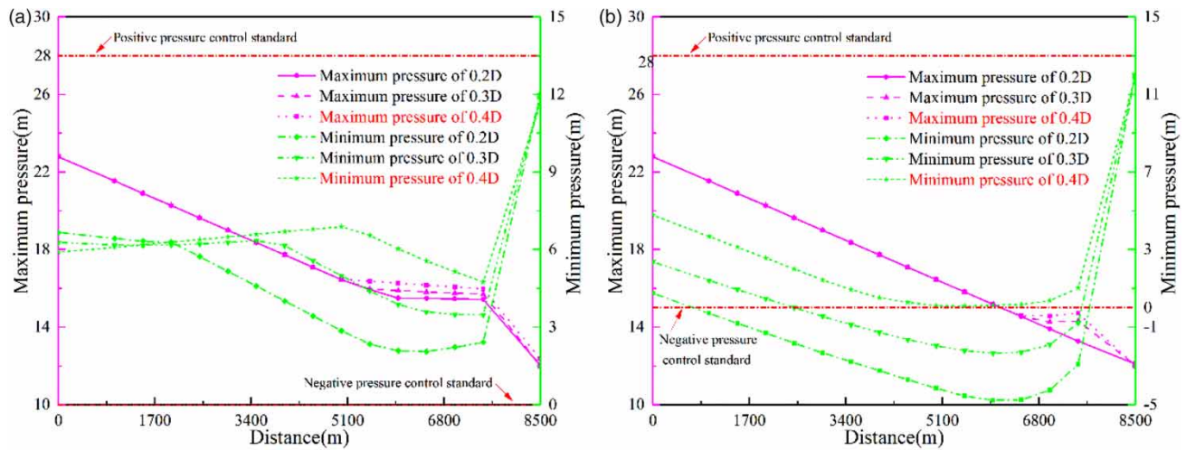
Figure 8 | Maximum and minimum pressure envelope of water supply system.
