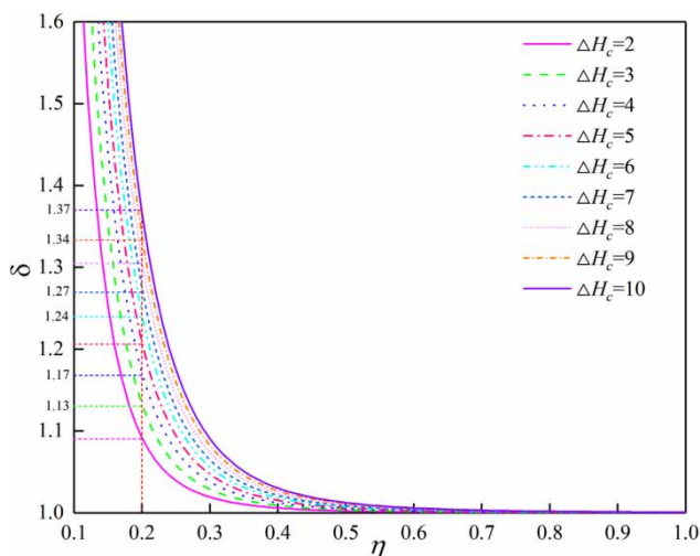
Figure 3 | The relationship between the loss ratio and the impedance hole diameter ratio under different pressure drop differences.
