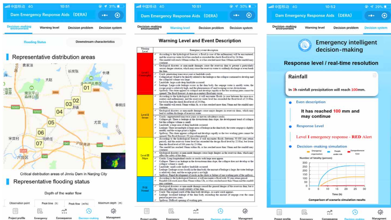
Figure 13 | The mobile APP interface of Dam Emergency Response Aids (DERA).
