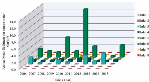
Figure 7 | Annual sediment inflow per sub-basins (per square meter).
