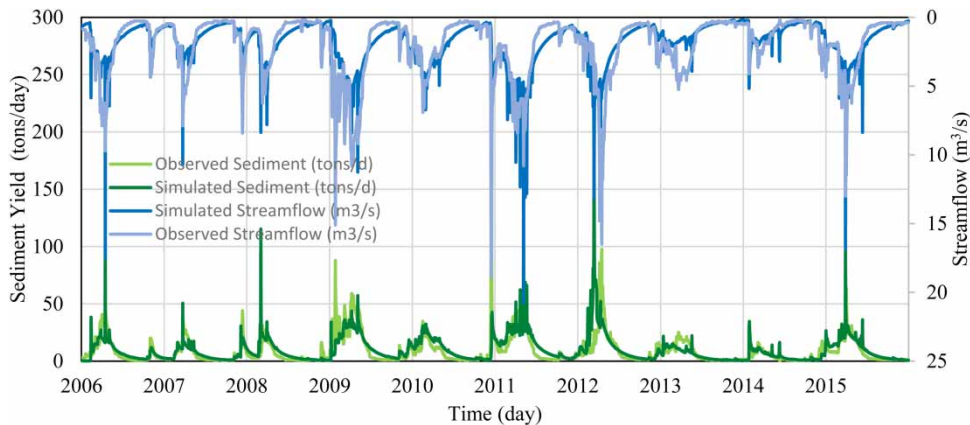
Figure 6 | Observed and simulated streamflow and sediment yield in the model calibration and validation period.
