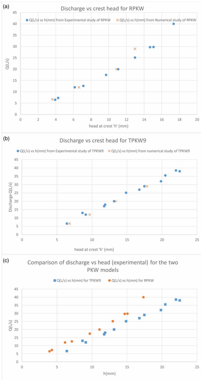
Figure 2 | (a) Comparison of an experimental and numerical study of discharge vs. head at the crest for RPKW. (b) Comparison of an experimental and numerical study of discharge vs. head at the crest for TPKW9. (c) Comparison of experimental discharge vs. head at the crest for RPKW and TPKW9.
