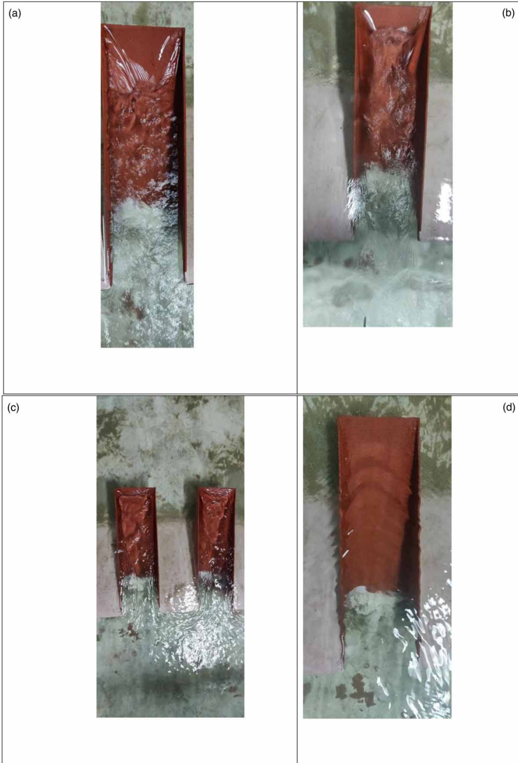
Figure 4 | Different stages in submergence of the outlet of RPKW.
