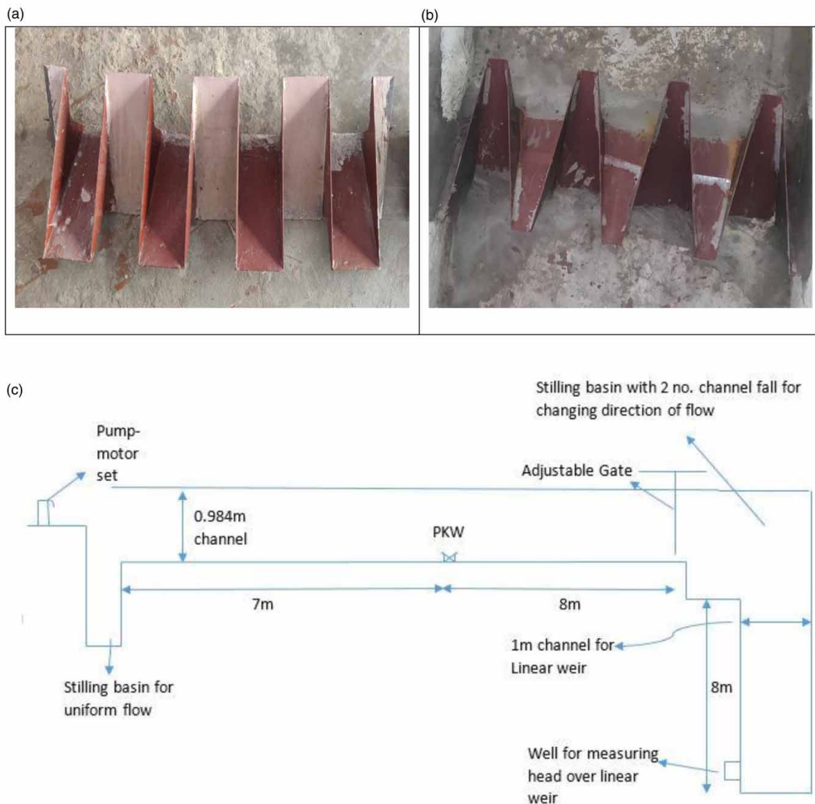
Figure 1 | Models used in the experimental study (a) RPKW, (b) TPKW9 and (c) experimental setup.
