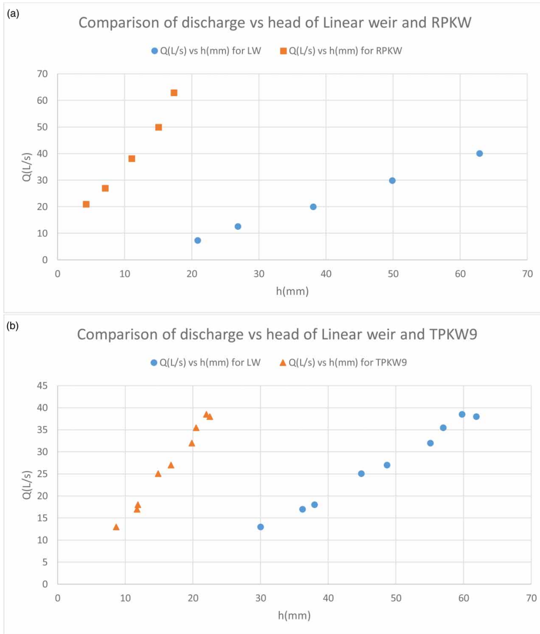
Figure 3 | (a) Comparison of experimental discharge vs. head at the crest for RPKW with that of a linear weir. (b) Comparison of experimental discharge vs. head at the crest for TPKW9 with that of a linear weir.
