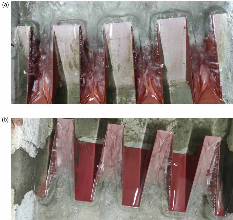
Figure 5 | Continuous water film in PKWs under partial submergence. (a) Continuous water film running around inlet-outlet of RPKW. (b) Continuous water film running around inlet-outlet of TPKW9.
