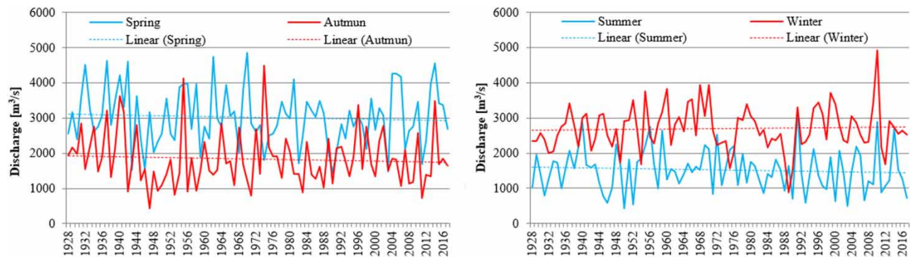
Figure 6 | Seasonal maximum discharge series at the Sremska Mitrovica gauging station (the Sava River) for spring, autumn, summer, and winter, respectively.
