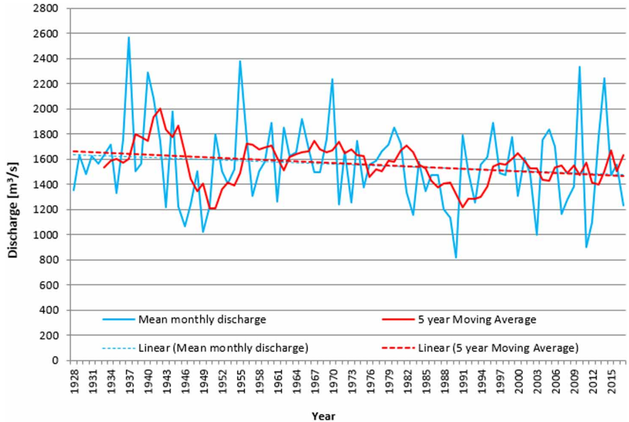
Figure 5 | The mean monthly discharge values with the linear trend line indicating the negative trend and the 5-year moving average for Sremska Mitrovica station for the 1928–2017 period.
