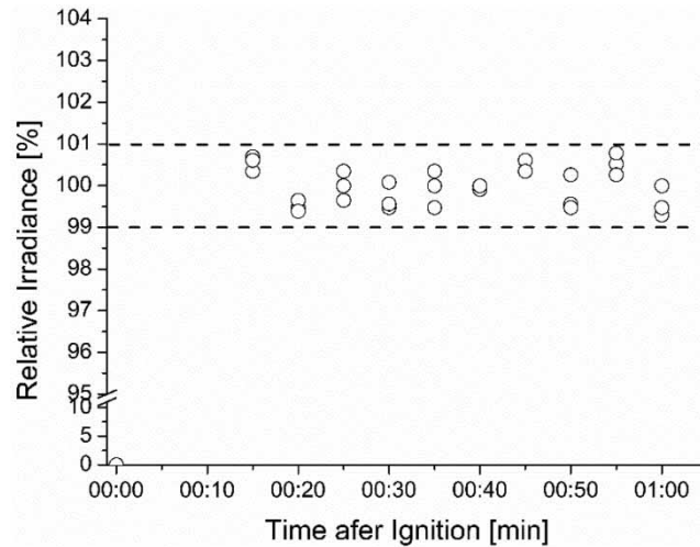
Figure 7 | Relative irradiance of an LP-lamp measured during 1 hour after ignition at a water temperature of 10.0 °C \pm 0.1 °C at approximately 1/3 of the lamp's length from its end.
