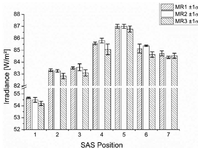
Figure 8 | Three different measurement runs (MR1, MR2, MR3) of irradiance along the length of a lamp made at SAS positions 1 to 7 during a day (at 20\text{ }^{\circ}\text{C} \pm 0.1\text{ }^{\circ}\text{C} ). Error bars indicate the standard deviation of measurements.
