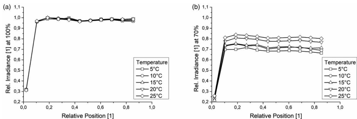
Figure 5 | Relative irradiance along an ALPHO lamp (length L = 1,200 mm) with a nominal power of 220 W in water at temperatures between 5 and 25 °C at full (a) and at 70% (b) ballast power.
