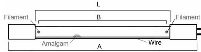
Figure 3 | Schematics of an amalgam-LP-high-output lamp, whereas A denotes the total length of the lamp, L the length of the uncovered glass bulb and B the distance between the spiral-wound filaments. In some lamps, the ends of the glass bulb and in some lamps also the filaments are hidden by the socket. In the last case: B > L .
