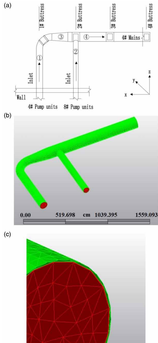
Figure 1 | (a) Schematic diagram of the pressure pipeline layout of Phase I's No. 2 pumping station; No. 1 pressure pipeline model mesh illustration showing (b) the integral structure and (c) a detail view.
