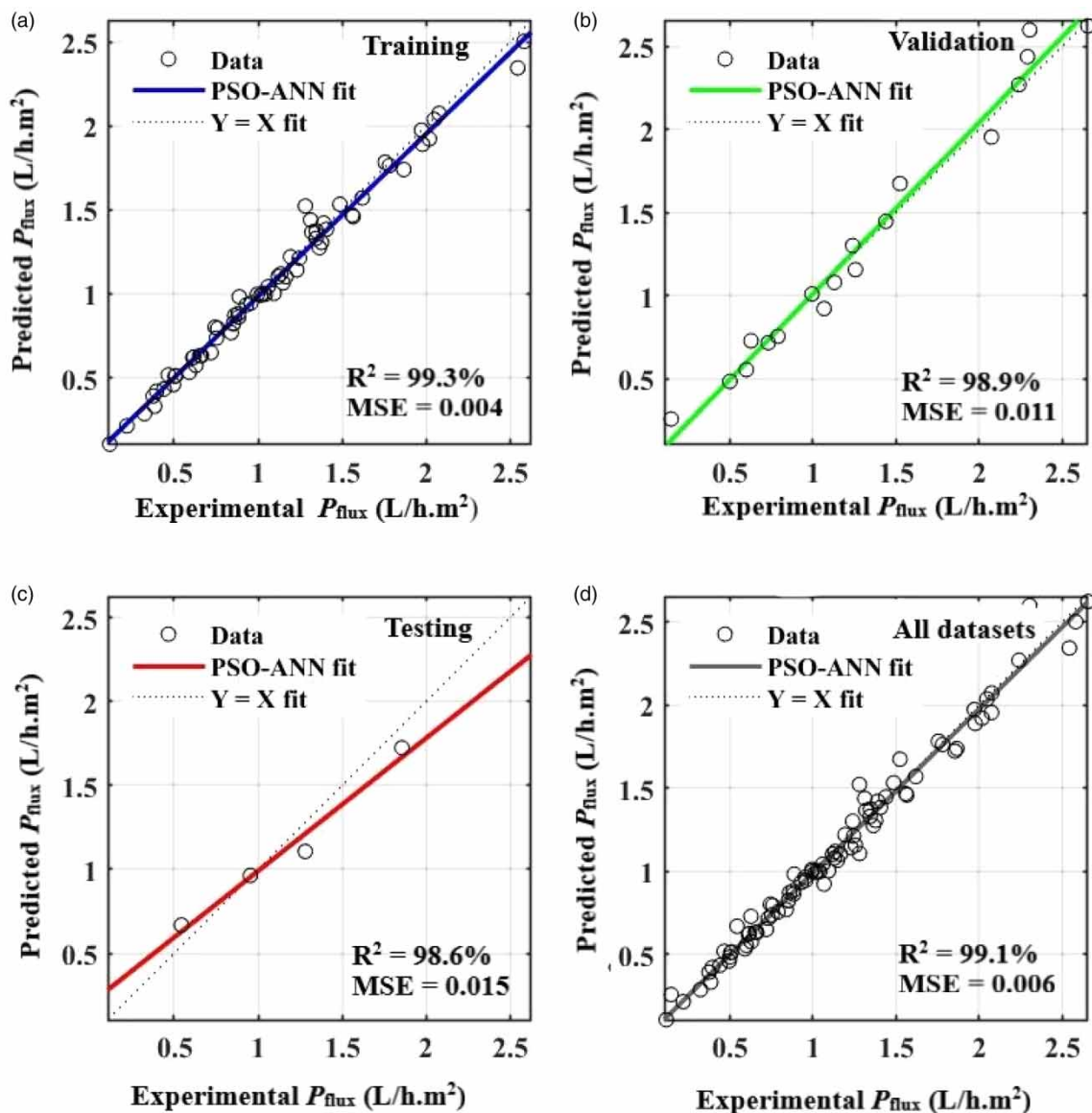
Figure 4 | Scatter plots of the predicted permeate flux ( P_{\text{flux}} (L/h.m 2 ) from the PSO-ANN (Model - 3): (a) training (75%), (b) validation (20%), (c) testing (5%), and (d) all datasets (100%).
