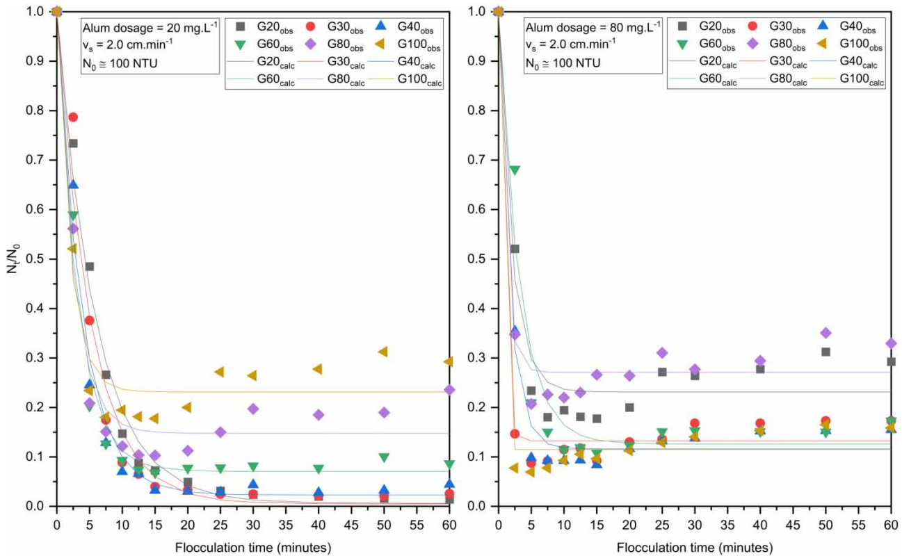
Figure 5 | Left: Model fitting to N_t/N_0 results with 20 \text{ mg}\cdot\text{L}^{-1} of alum. Right: Model fitting to N_t/N_0 results with 80 \text{ mg}\cdot\text{L}^{-1} of alum. All assays performed with high-turbidity raw water ( \approx 100 \text{ NTU} ), all \bar{G} values and 2.0 \text{ cm}\cdot\text{min}^{-1} of settling velocity.
