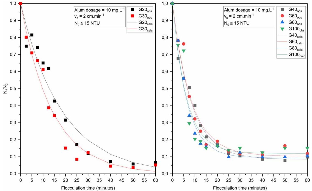
Figure 1 | Left: Model fitting to N_t/N_0 results with \bar{G} values of 20 and 30 s^{-1} . Right: Model fitting to N_t/N_0 results with \bar{G} values of 40, 60, 80, and 100 s^{-1} . All results with low-turbidity raw water ( \approx 15 NTU), 10 mg \cdot L^{-1} of alum and 2.0 cm \cdot min^{-1} of settling velocity.
