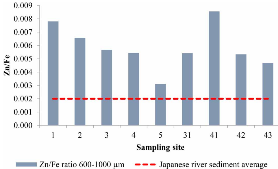
Figure 7 | Normalized ratios of Zn concentration in surface sediment of grain size 600–1,000 µm using Fe as conservative element. Japanese river sediment average ( Gamo 2007 ) data have been considered as baseline values (broken lines).
