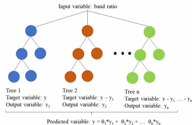
Figure 2 | The construction process of GBRT model.
