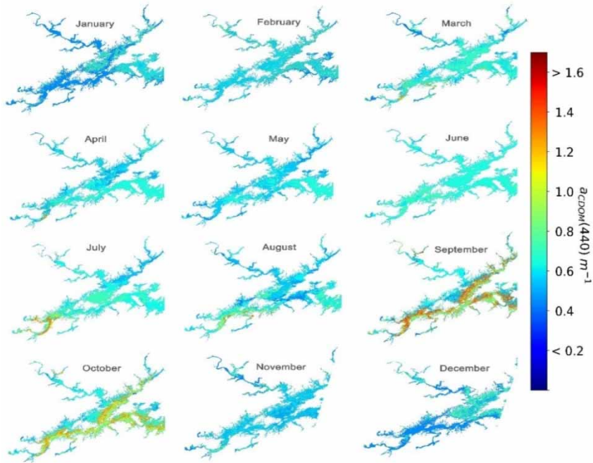
Figure 6 | Monthly estimated CDOM concentrations observed from Sentinel-2 images in Xin'anjiang Reservoir in 2018.
