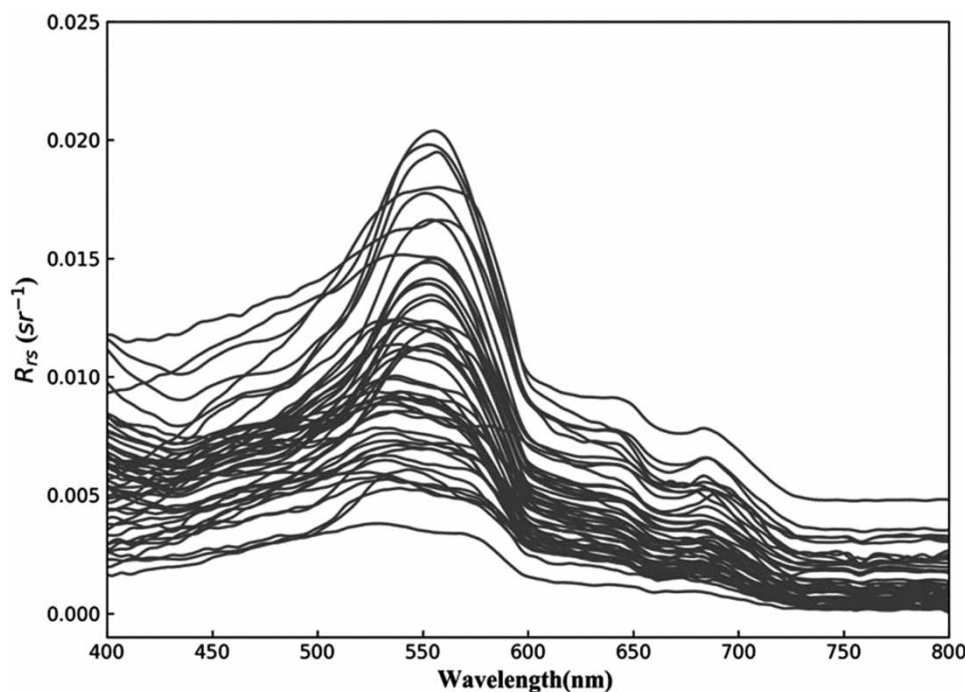
Figure 3 | The field measured above-surface spectra ( R_{rs} ) in Xin'anjiang Reservoir.
