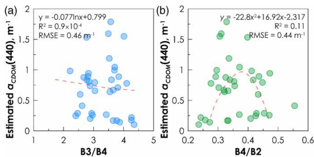
Figure 5 | Testing two previous empirical models to retrieve the low CDOM concentrations in Xin'anjiang Reservoir.
