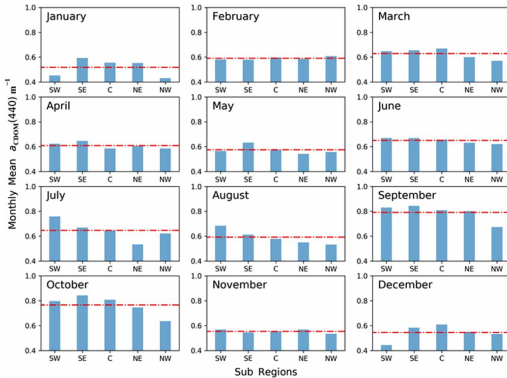
Figure 7 | Estimated monthly mean a_{CDOM}(440) derived from Sentinel-2 images in five sub-regions of Xin'anjiang Reservoir. The red lines represent the mean values of the entire reservoir. All subfigures have the same labels and axes as the subfigure of January.
