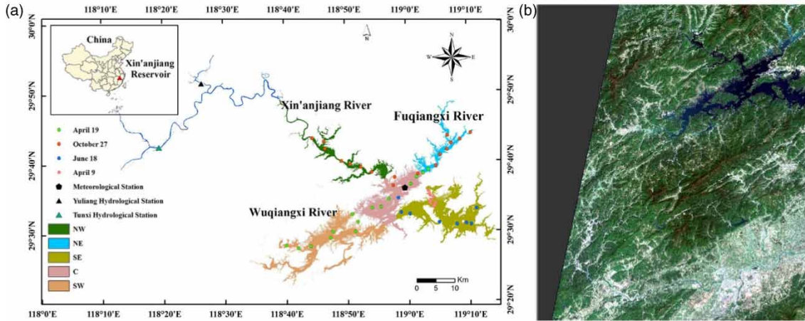
Figure 1 | (a) Study site map showing the field sampling points, locations of meteorological stations and hydrological stations, three main inflow rivers, and five sub-regions (C, NE, NW, SE, and SW) in Xin'anjiang Reservoir. (b) A Sentinel-2 raw image acquired on April 9 in 2018, showing the land cover in the watershed of the Xin'anjiang Reservoir.
