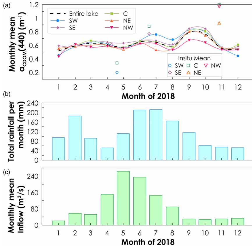
Figure 8 | (a) The image-estimated and field measured CDOM temporal variations (smoothed) in five sub-regions as well as the entire Xin'anjiang Reservoir, (b) monthly total precipitation in Xin'anjiang Reservoir in 2018, and (c) monthly mean inflow rate from the Xin'anjiang River in 2018.
