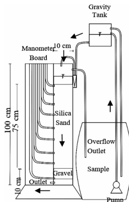
Figure 1 | Rapid-sand filter reactor scheme.
