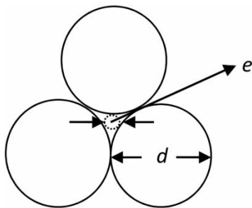
Figure 9 | The diameter of the opening between the filter media pores (Huisman & Wood 1974).
