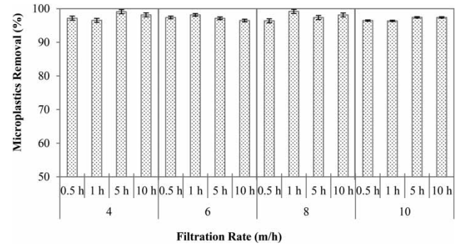
Figure 5 | Microplastics removal (plastic flakes) using filter media ES 0.39 mm.
