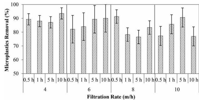
Figure 8 | Microplastics removal (tyre flakes) using filter media ES 0.68 mm.
