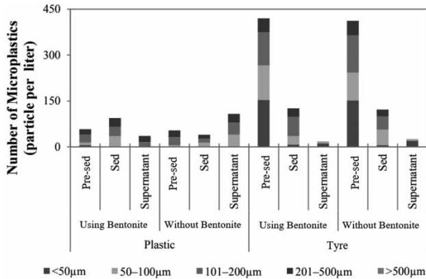
Figure 4 | Size distribution and number of microplastics.
