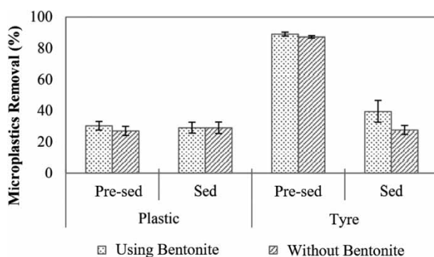
Figure 3 | Microplastics percentage removal.
