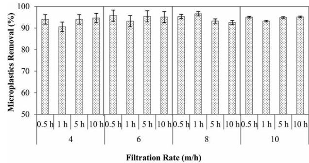
Figure 7 | Microplastics removal (plastic flakes) using filter media ES 0.68 mm.
