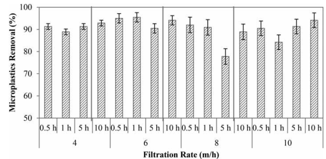
Figure 6 | Microplastics removal (tyre flakes) using filter media ES 0.39 mm.
