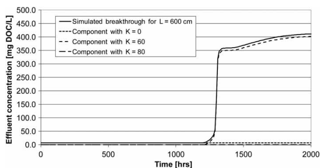
Figure 6 | Predicted breakthrough curve of pre-treated HTC spent grains process water in a technical-scale GAC column; conditions: bed length 6 m (3 columns in series), empty bed contact time 7.5 hours, influent concentration 420 mg DOC/L.
