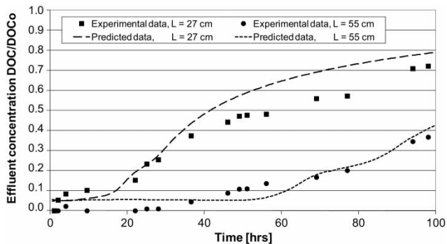
Figure 5 | Experimental and predicted breakthrough curves of pre-treated HTC food leftovers process water.
