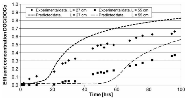
Figure 3 | Experimental and predicted breakthrough curves of pre-treated HTC spent grains process water.
