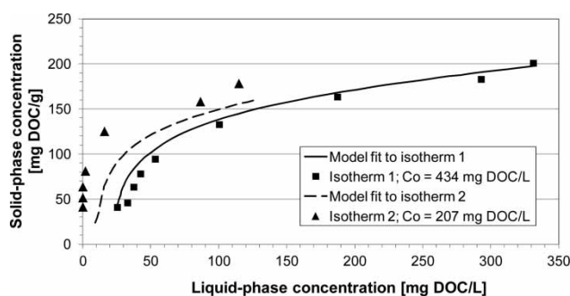
Figure 1 | Adsorption isotherms of pre-treated HTC food leftovers process water and fit of the IAST model.
