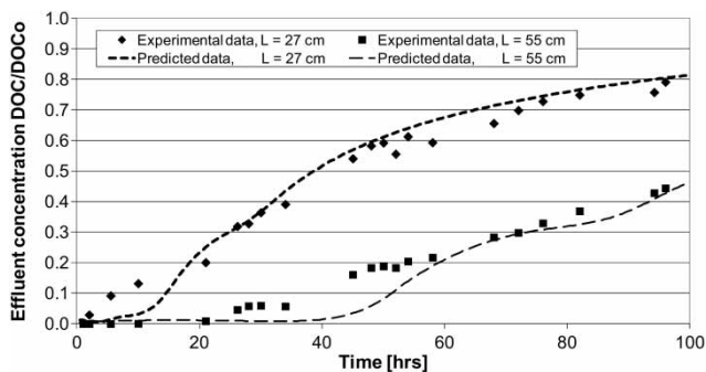
Figure 4 | Experimental and predicted breakthrough curves of pre-treated HTC sugar beet residuals process water.
