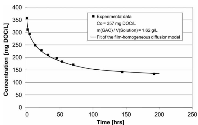
Figure 2 | Adsorption rate curve of pre-treated HTC food leftovers process water on granular Norit ROW 0.8 S.
