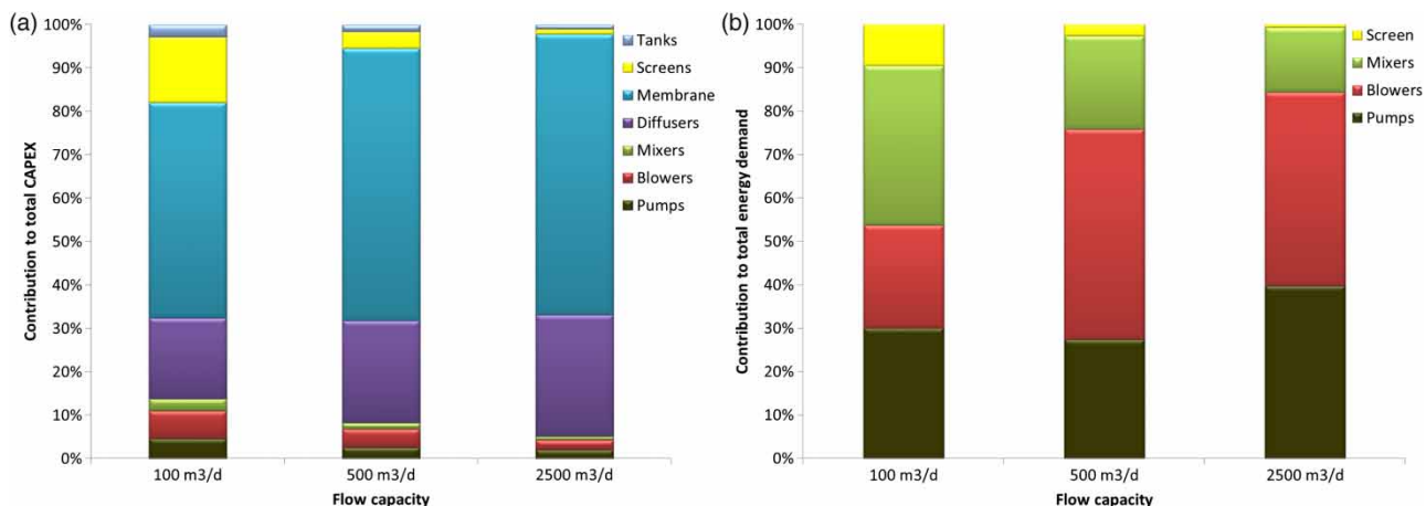
Figure 3 | (a) Capital cost and (b) energy demand contributions at the three different flow capacities.
