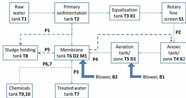
Figure 2 | Plant schematic; see Table 1 for codes.
