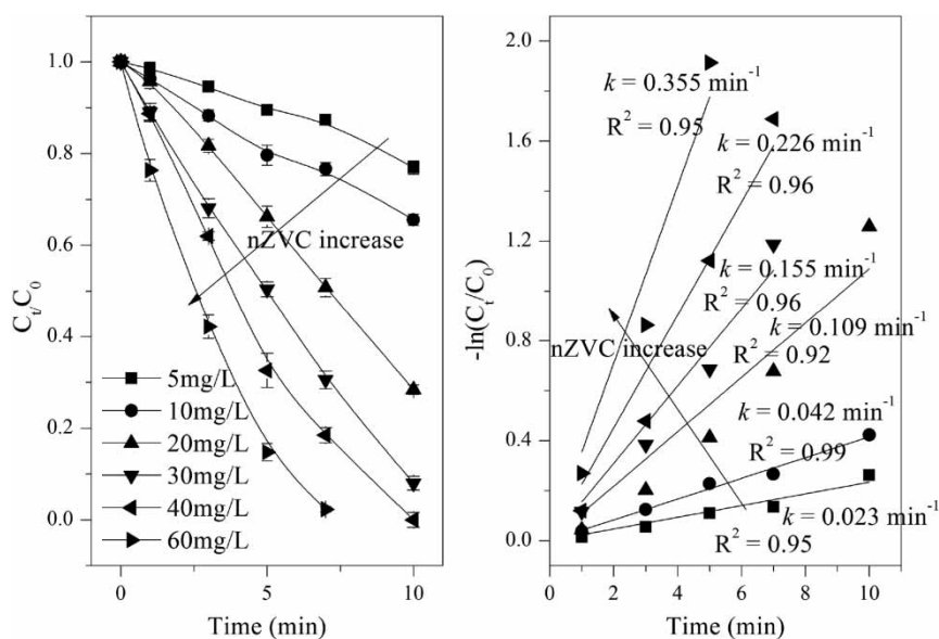
Figure 8 | Effect of nZVC dosage on BA degradation in the nZVC/PMS process. [BA]_0 = 20 \mu\text{M} , [PMS]_0 = 1 \text{ mM} , [nZVC]_0 = 5, 10, 20, 30, 40, \text{ and } 60 \text{ mg/L} , \text{pH}_0 = 3.0 .
