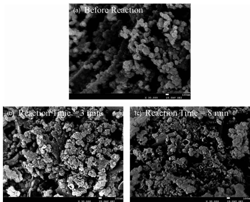
Figure 4 | SEM images of nZVC before (a) and after (b and c) reaction in nZVC/PMS process.
