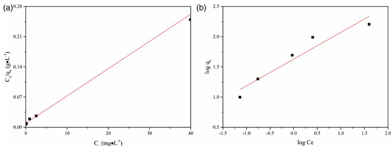
Figure 5 | Isotherm plots for adsorption of MB onto LSP: (a) Langmuir and (b) Freundlich isotherm.
