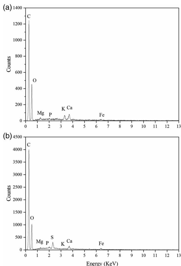
Figure 2 | EDS spectrum of LSP (a) before and (b) after adsorption of MB.
