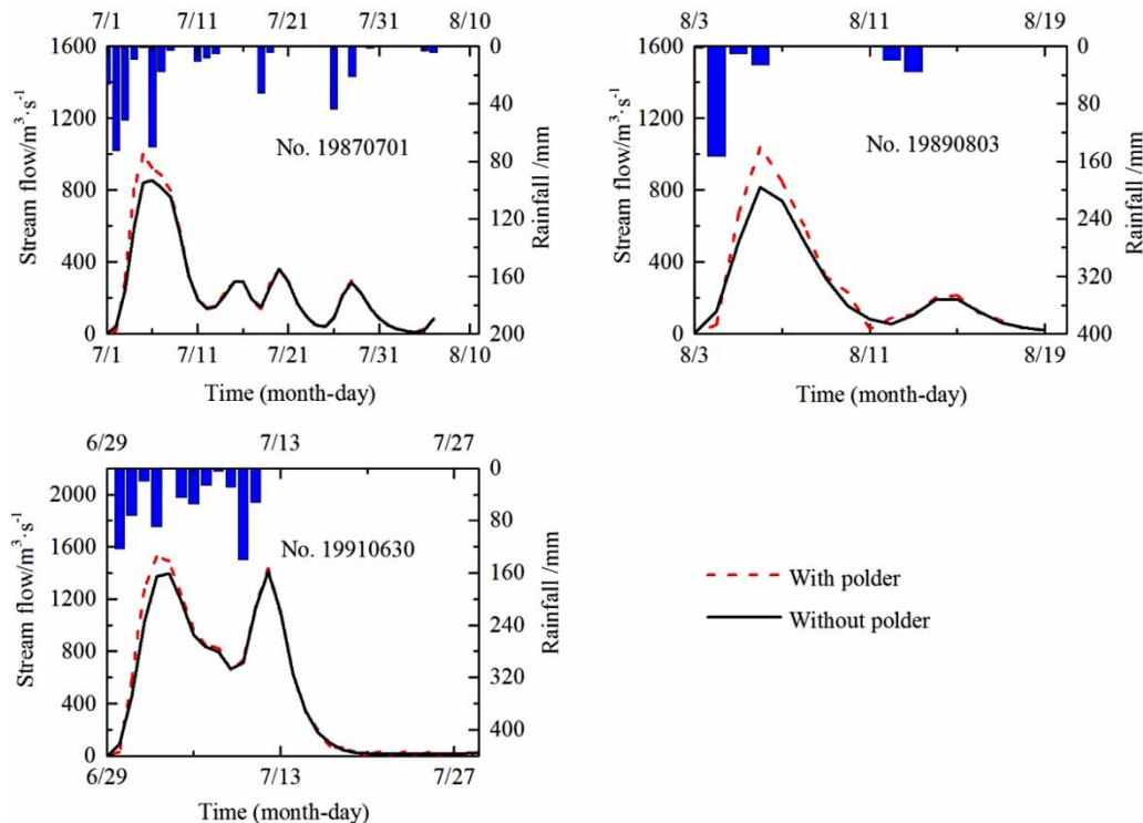
Figure 4 | Comparison of stream flows of flood control pattern with the urban agglomeration polders and without polders for flood events.
