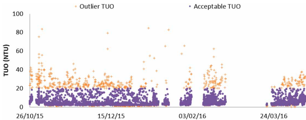
Figure 4 | Turbidity outlet (TUO) by plant dosage at SRA WWTP. Outlier TUO (crosses) and Acceptable TUO (circles).
