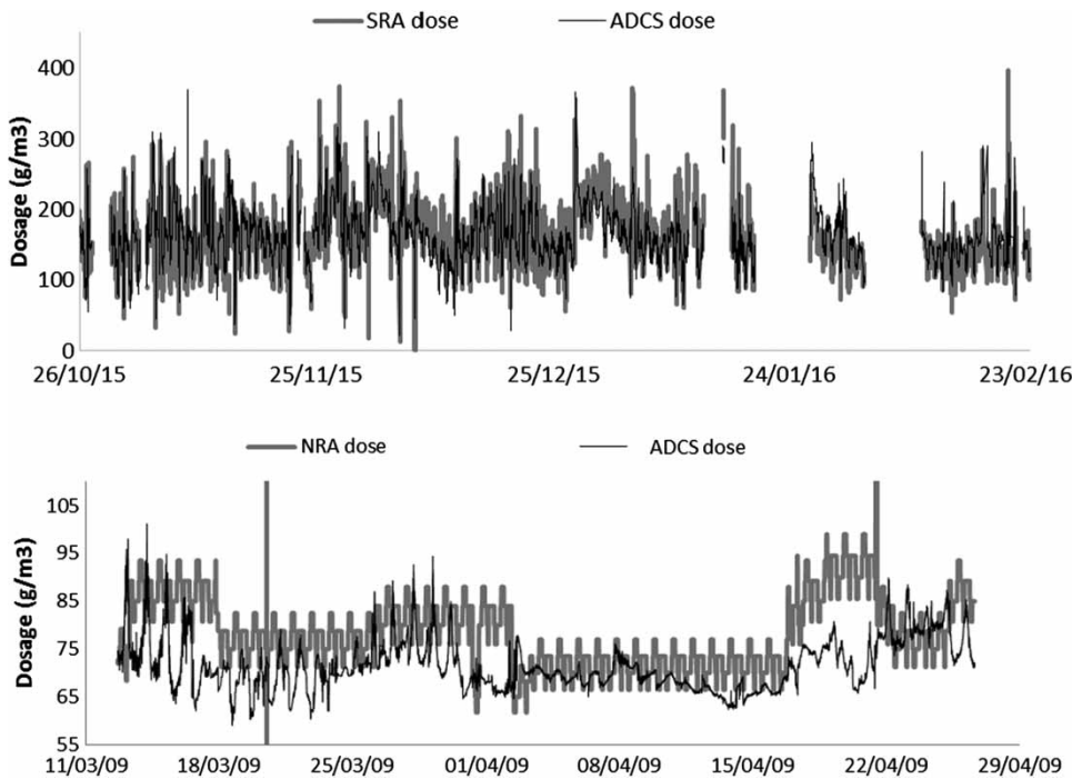
Figure 2 | Traditional flow proportional WW dosing methods at SRA (above) and NRA (below) compared with the ADCS predictions, a comparison during the testing period without active dosing.
