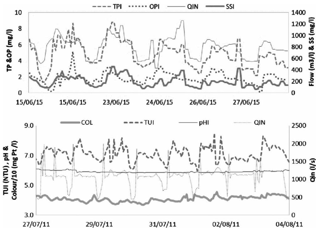
Figure 1 | Variations of influent water quality of SRA WWTP (above) and Vansjø DWTP (below): colour inlet (mg Pt/L), influent flow (L/s), turbidity (NTU), influent pH, influent Ortho-P (mg P/L), influent Total-P (mg P/L) and suspended solids (mg/L).
