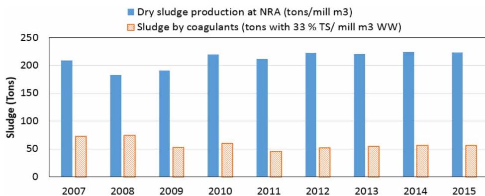
Figure 6 | Comparison of annual unit dry sludge production with the calculated sludge production (33%) by coagulants (VA-Support 2012).
