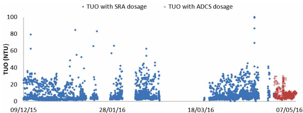
Figure 5 | The TUO with SRA dosage (crosses) and TUO with ADCS (circles).
