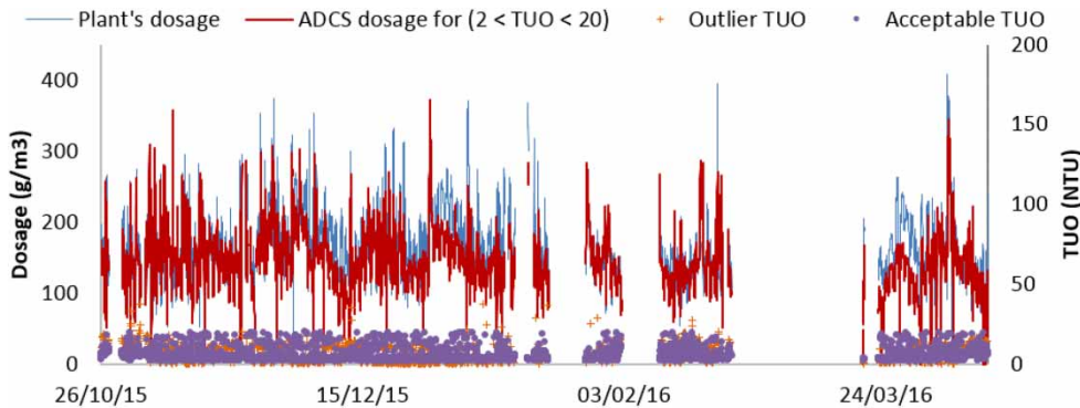
Figure 3 | Comparison between plant's dosage and the ADCS dose predictions to obtain TUO between 2 and 20 NTU. Outlier TUO (crosses) and Acceptable TUO (circles).
