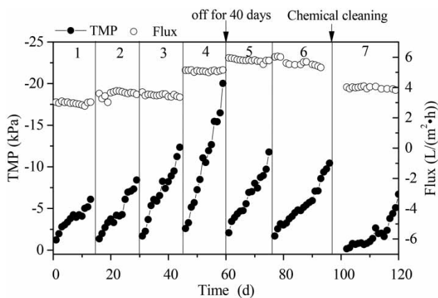
Figure 5 | TMP and membrane flux variation under different operation conditions.
