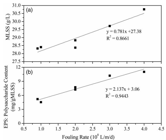
Figure 6 | Relationship between the fouling rate and both mixed liquor suspended solids (MLSS) and the polysaccharide content of the EPS.
