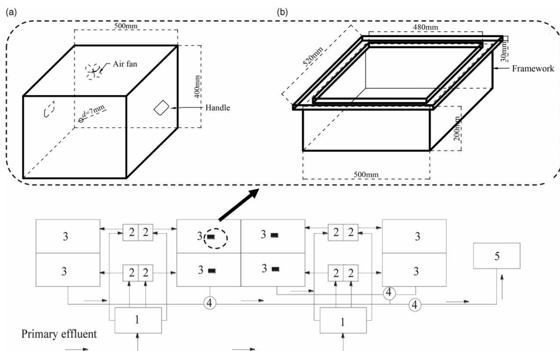
Figure 2 | Sketch showing of the SWI system and static chambers. (a) Box. (b) Foundation support.
