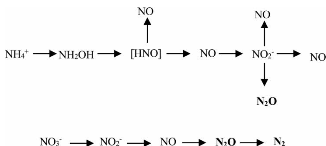
Figure 1 | N 2 O production mechanisms in SWI system.
