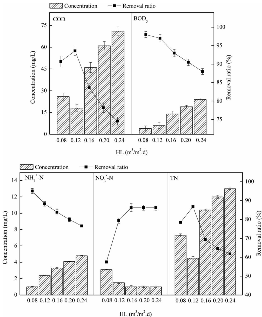
Figure 3 | The variation of effluent quality under different HLs.
