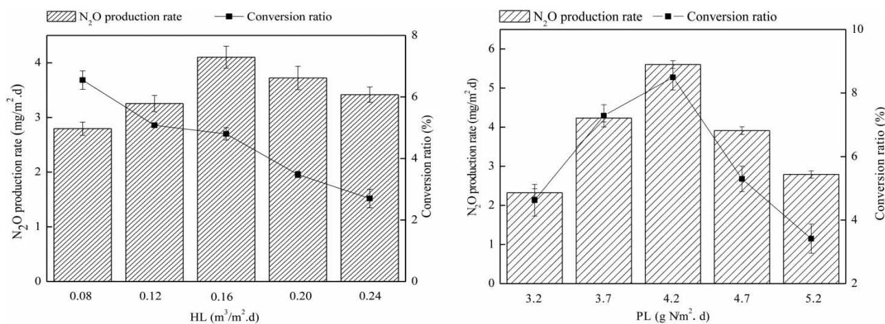
Figure 4 | The variation of N 2 O production rate and conversion ratio under HL (a) and PL (b).
