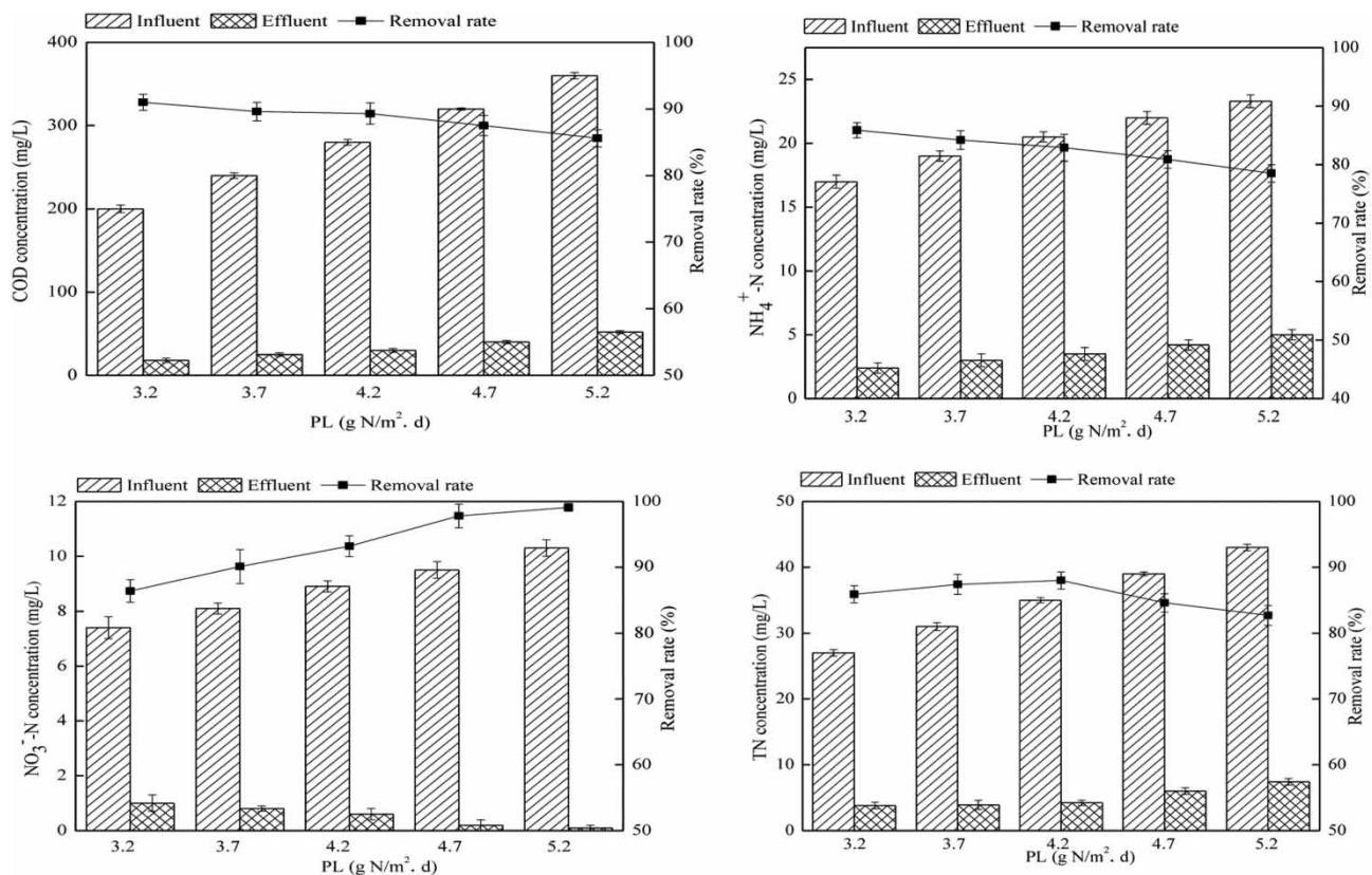
Figure 5 | The variation of removal efficiency under different PLs.
