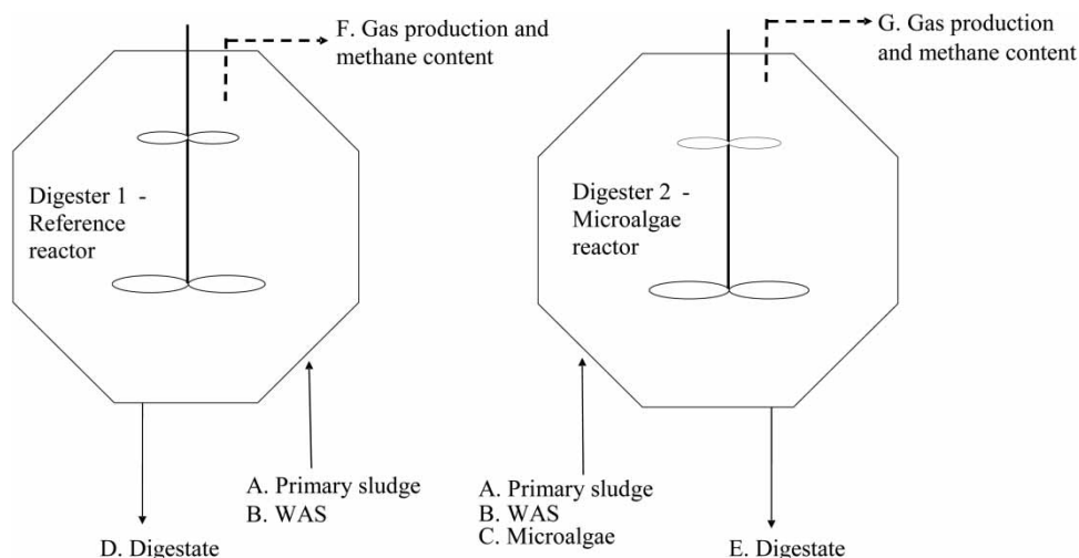
Figure 2 | Semi-continuous pilot digesters.
