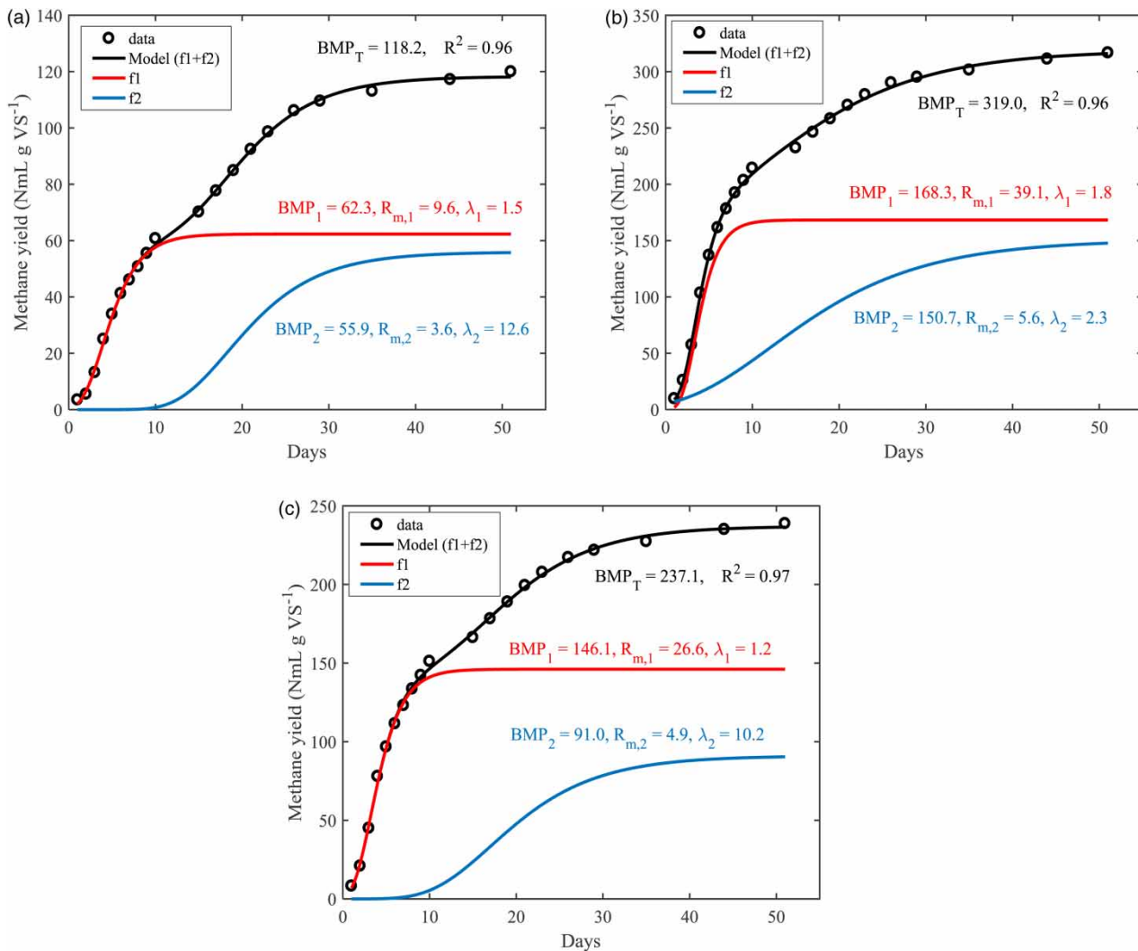
Figure 4 | Kinetic model (cf. Equation (8), black line) and experimental data (circles) for (a) 100% microalgae, (b) 100% sewage sludge, and (c) 58% sewage sludge and 42% microalgae. Parameters ( BMP_1 , R_{m,1} , \lambda_1 ) refer to the function f1 (red line), parameters ( BMP_2 , R_{m,2} , \lambda_2 ) refer to the function f2 (blue line). BMP_T = BMP_1 + BMP_2 . Please refer to the online version of this paper to see this figure in colour: http://dx.doi.org/10.2166/wst.2017.583 .
