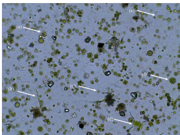
Figure 3 | Microalgae present in the substrate. (a) Scenedesmus sp., (b) Ankistrodesmus sp., (c) Chlorella sp., (d) Scenedesmus opoliensis , (e) Scenedesmus quadricauda , (f) Coelastrum sp., magnification: \times 200 . Illustration: F. Gentili.
