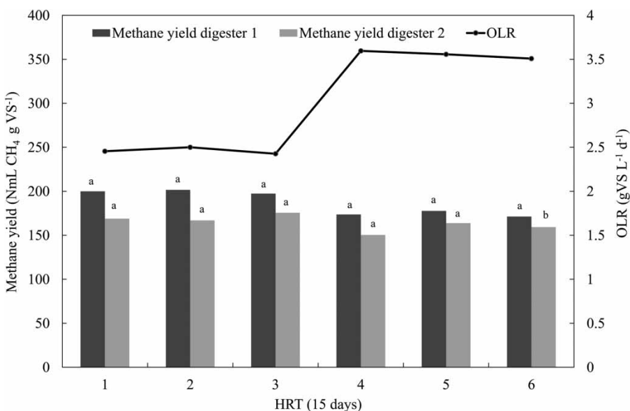
Figure 5 | Methane yield per incoming g VS for digester 1 (Reference digester) and digester 2 (Experimental digester). Statistically significant differences ( p = 0.05 ) are indicated by different letters. The statistical analysis only compared the two digesters for each HRT and did not address differences between HRTs.
