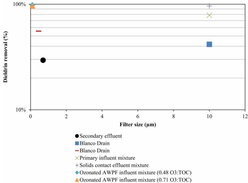
Figure 7 | Dieldrin removal through filtration as a function of filter size and water quality.
