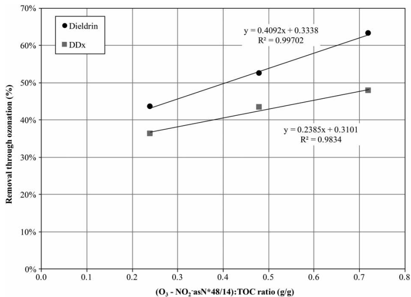
Figure 5 | Impact of ozone to total organic carbon ratio on dieldrin and DDX removal in the Blanco Drain-Regional Treatment Plant effluent mixture.
