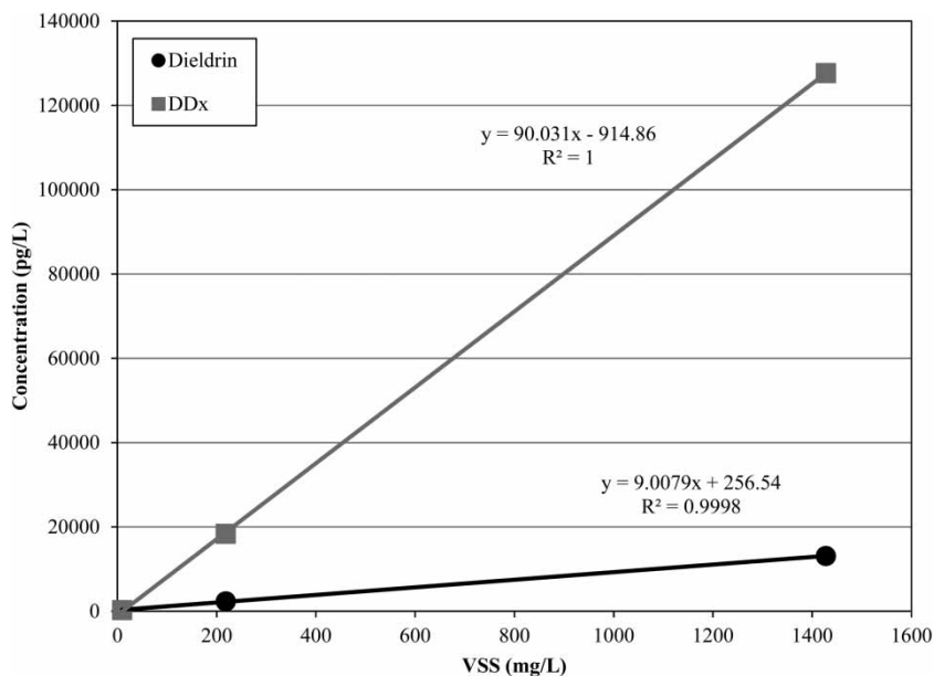
Figure 3 | Relationship between volatile suspended solids and dieldrin and DDX in the Regional Treatment Plant.
