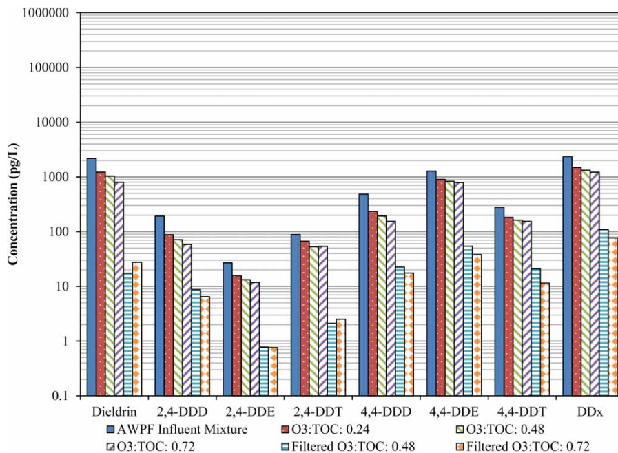
Figure 6 | Dieldrin and DDX removal through membrane filtration of the Blanco Drain-Regional Treatment Plant effluent mixture.
