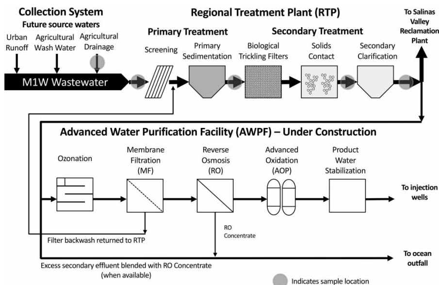
Figure 1 | Process flow schematic of the Regional Treatment Plant, the Advanced Water Purification Facility, and the future source waters, with sampling locations indicated.
