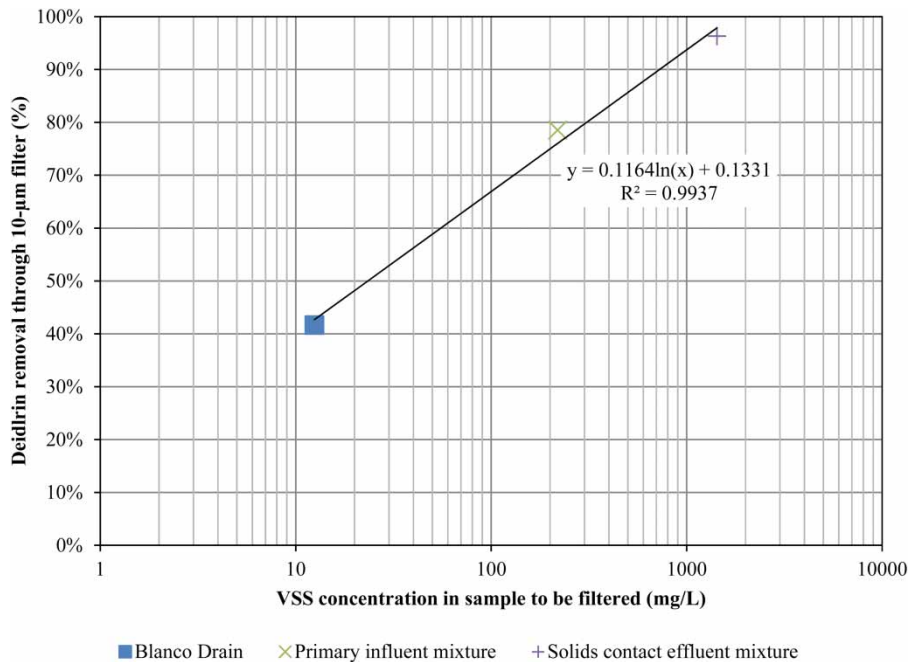
Figure 8 | 10- \mu\text{m} filter removal of dieldrin as a function of volatile suspended solids.
