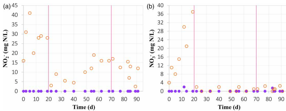
Figure 7 | Nitrite (a) and nitrate (b) concentration in the influent (●) and effluent (○) over time, for the 6 h anoxic-aerobic-anoxic cycle with addition of methanol.
