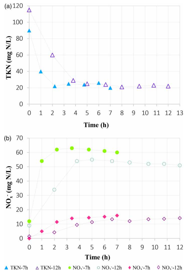
Figure 2 | (a) Profile of TKN concentration during aeration, (b) profile of nitrite and nitrate concentration during aeration.
