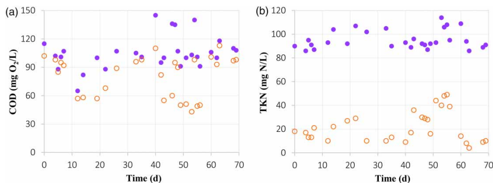
Figure 4 | COD (a) and TKN (b) concentration in the influent (●) and effluent (○) over time, for the 6 h aerobic/anoxic cycle.
