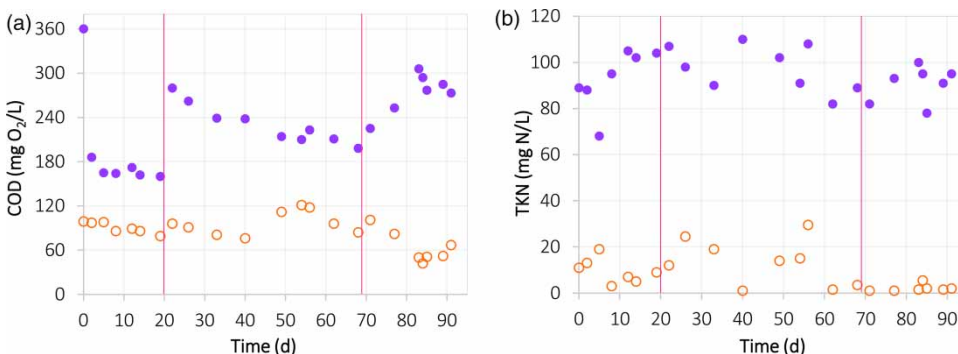
Figure 6 | COD (a) and TKN (b) concentration in the influent (●) and effluent (○) over time, for the 6 h anoxic-aerobic-anoxic cycle with addition of methanol.
