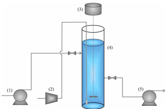
Figure 1 | Scheme of the SBR plant. (1) Filling pump, which supplies the wastewater from the anaerobic treatment to the reactor, (2) compressor, responsible for supplying the air for the aeration step, (3) mechanical stirrer, (4) SBR reactor, (5) pump that drains the water after treatment.
