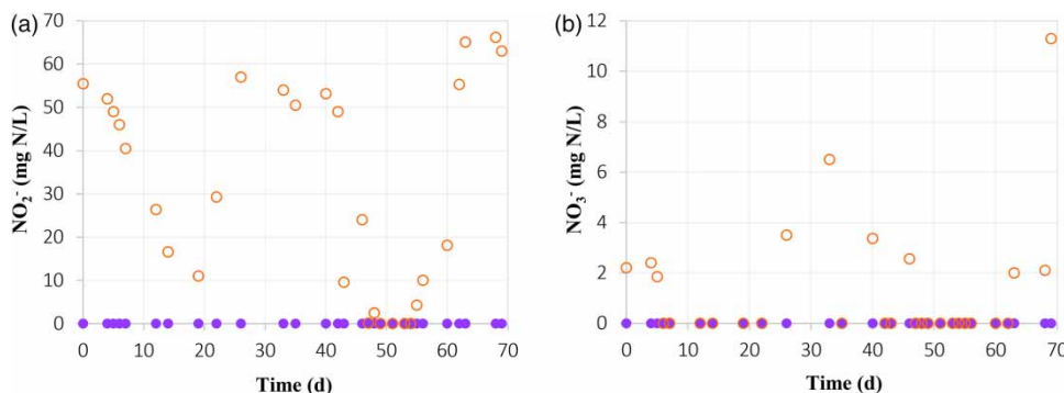
Figure 5 | Nitrite (a) and nitrate (b) concentration in the influent (●) and effluent (○) over time, for the 6 h aerobic/anoxic cycle.
