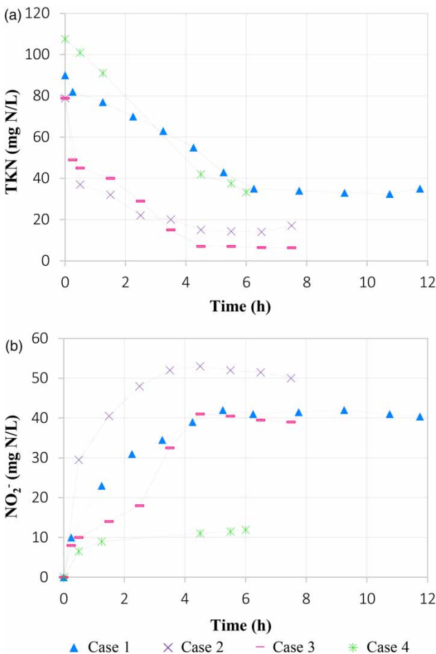
Figure 3 | Profiles of TKN (a) and \text{NO}_2^- (b) concentrations over time for the different cycles.
