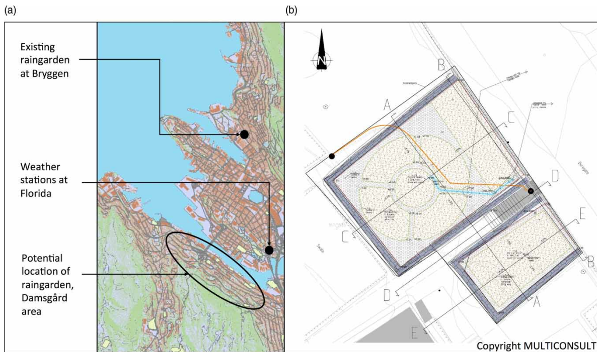
Figure 2 | Overview of the study site, showing the (a) location of existing raingarden at Bryggen, weather stations at Florida and study site Damsgård, and (b) layout of the existing raingarden at Bryggen.
