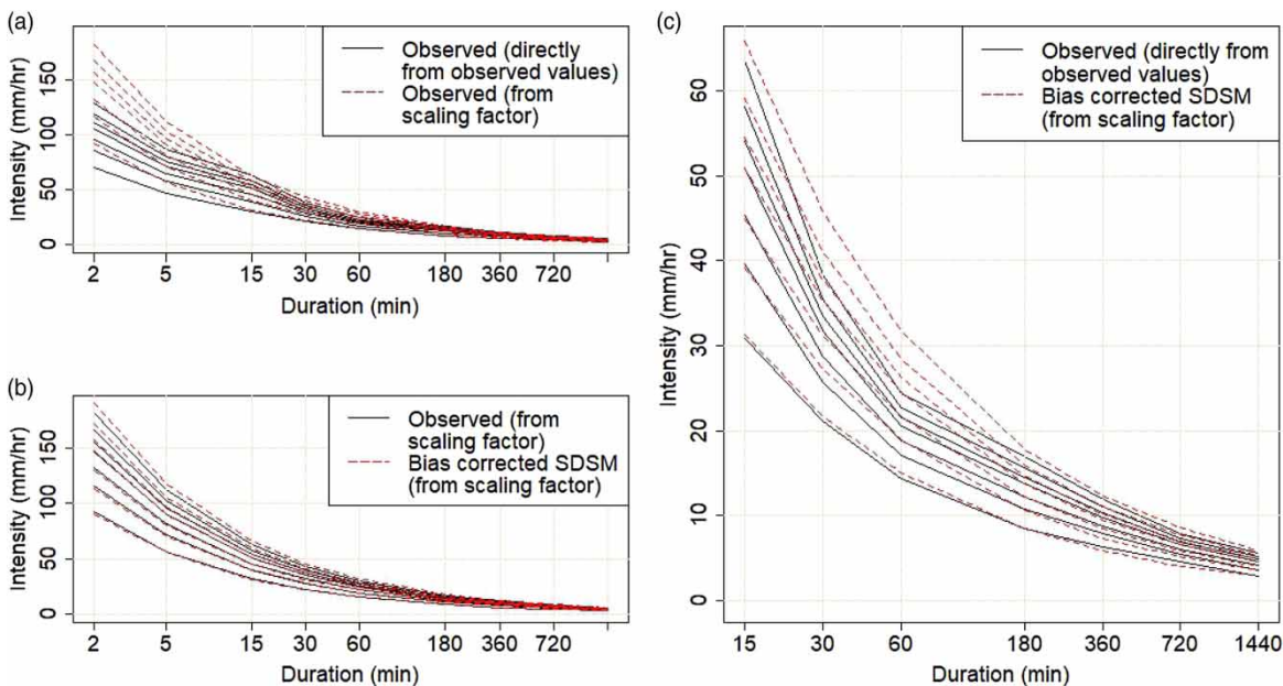
Figure 4 | IDF curves showing the ability of the applied methodology to represent historical precipitation intensities. (a) observed precipitation, derived directly from the observed values, and by using the scaling factor; (b) observed and bias corrected SDSM precipitation, both developed using the derived scaling factor; (c) observed precipitation found directly from observed values and bias corrected SDSM precipitation found by using the scaling factor. The return periods are 2, 5, 10, 20, 30, 50 and 100 years.
