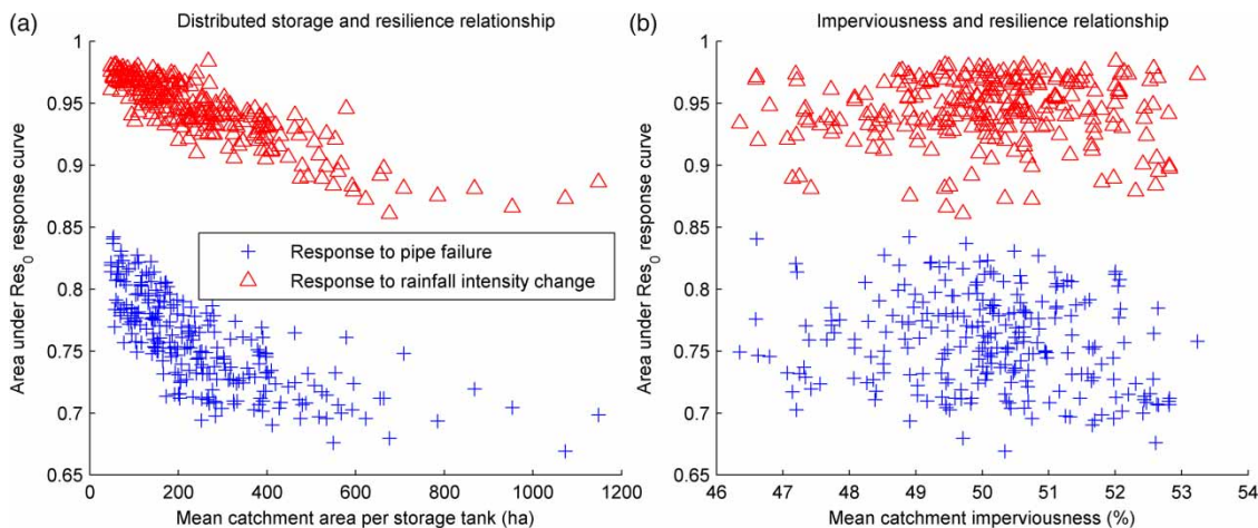
Figure 2 | Relationship between a performance-based resilience indicator, distributed storage and imperviousness in the VCSs before intervention.
