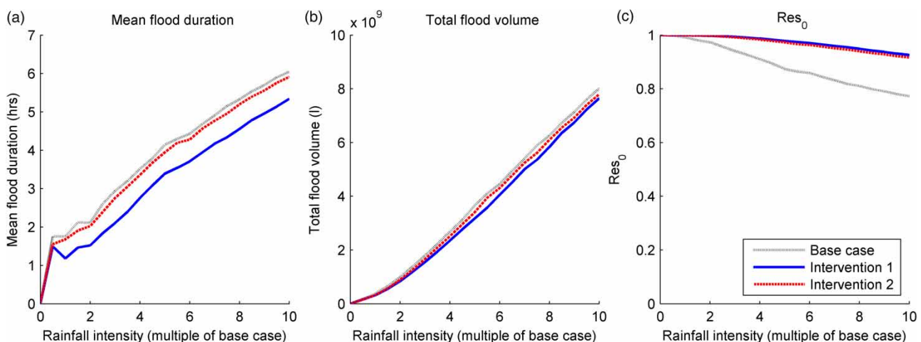
Figure 3 | Effect of interventions on response to increased rainfall in VCS 180.
