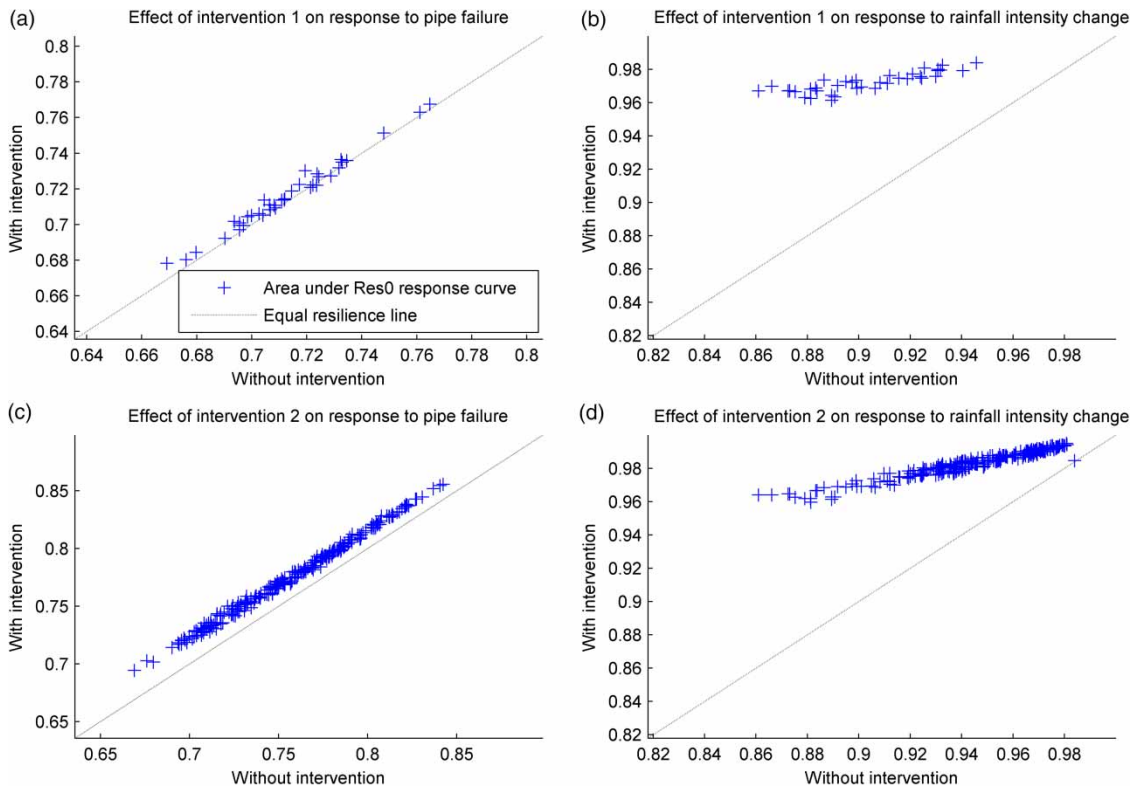
Figure 4 | Effect of interventions on performance-based resilience indicators; each cross represents one VCS.
