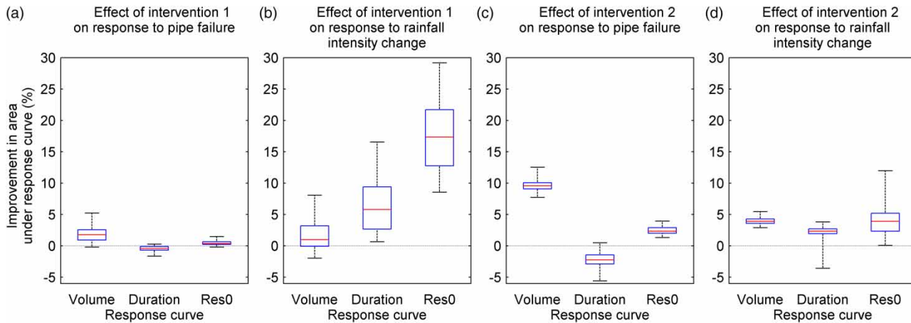
Figure 5 | Improvement in area under response curves for pipe failure and rainfall intensity change provided by interventions.
