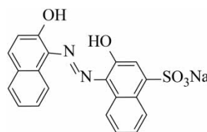
Figure 1 | Structure of Mordant Black 17.
