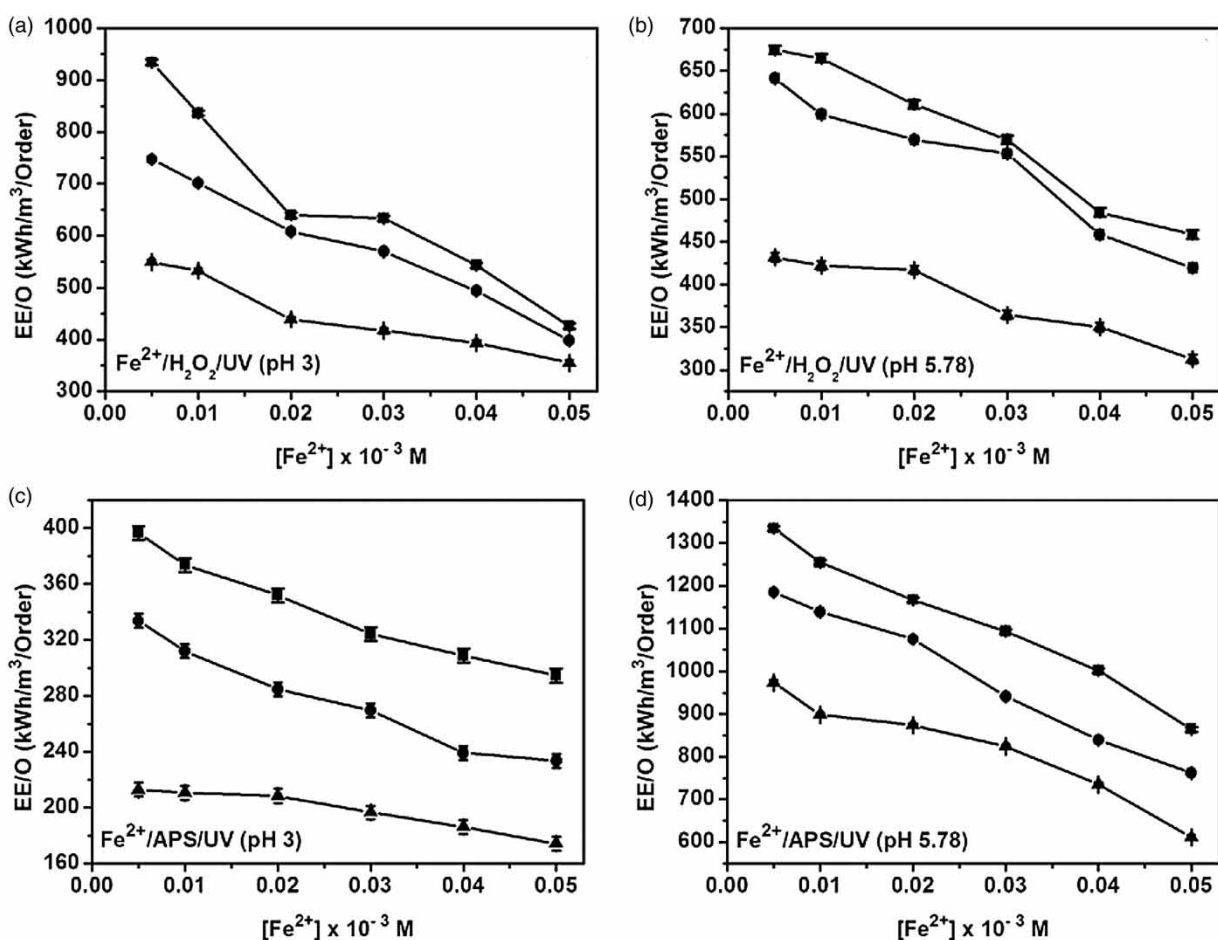
Figure 4 | Effect of \text{Fe}^{2+} and oxidant concentration on the EE/O values for treatment of MB 17 by \text{Fe}^{2+} /oxidant/UV systems: [MB 17] = 0.05 mM; oxidant concentration: -■- 0.35 mM; -●- 0.70 mM; -▲- 1.4 mM. A: UV intensity = 1,417 \mu\text{W cm}^{-2} , treatment period = 60 min; B: UV intensity = 1,064 \mu\text{W cm}^{-2} , treatment period = 60 min; C: UV intensity = 1,417 \mu\text{W cm}^{-2} , treatment period = 30 min; D: UV intensity = 1,417 \mu\text{W cm}^{-2} , treatment period = 90 min.
