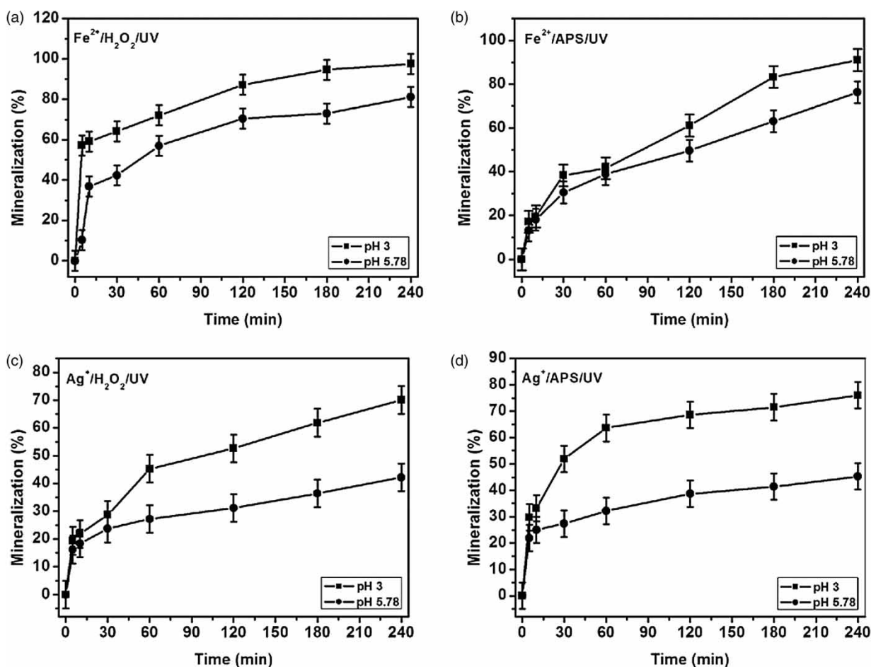
Figure 2 | Effect of pH on the mineralization of MB 17: [MB 17] = 0.05 mM; [M^{n+}] = 0.05 mM; [oxidant] = 0.35 mM; UV intensity = 213 \mu W cm^{-2} .
