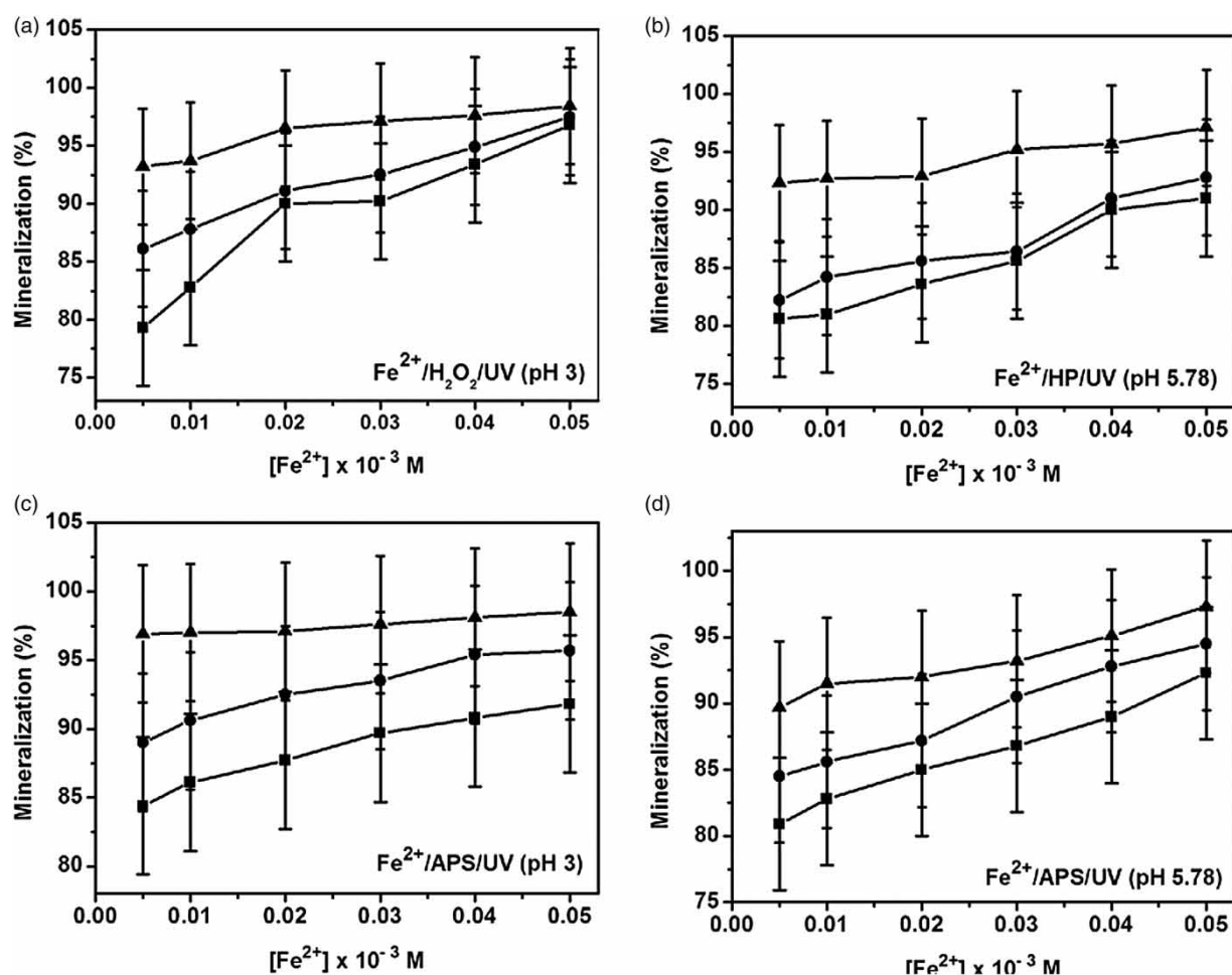
Figure 3 | Effect of \text{Fe}^{2+} and oxidant concentration on the mineralization of MB 17 by \text{Fe}^{2+} /oxidant/UV systems: [MB 17] = 0.05 mM; oxidant concentration: \blacksquare – 0.35 mM; \bullet – 0.70 mM; \blacktriangle – 1.4 mM. A: UV intensity = 1, 417 \mu\text{W cm}^{-2} , treatment period = 60 min; B: UV intensity = 1, 064 \mu\text{W cm}^{-2} , treatment period = 60 min; C: UV intensity = 1, 417 \mu\text{W cm}^{-2} , treatment period = 30 min; D: UV intensity = 1, 417 \mu\text{W cm}^{-2} , treatment period = 90 min.
