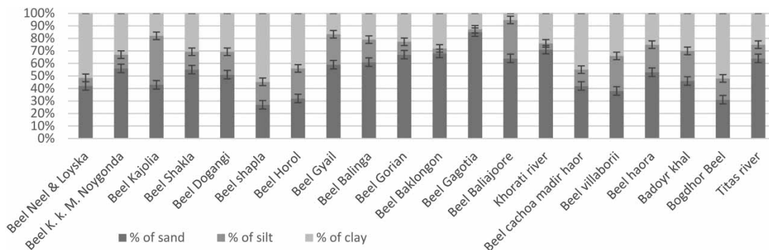
Figure 6 | Percentage of sand, silt and clay in different wetlands of Brahmanbaria district.
