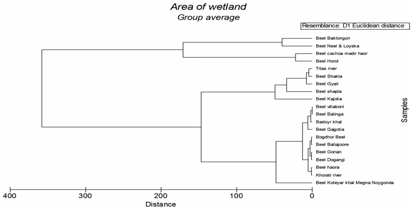
Figure 2 | Dendrogram constructed on the basis of area, showing the percentage of distance among different wetlands of Brahmanbaria district, Bangladesh.
