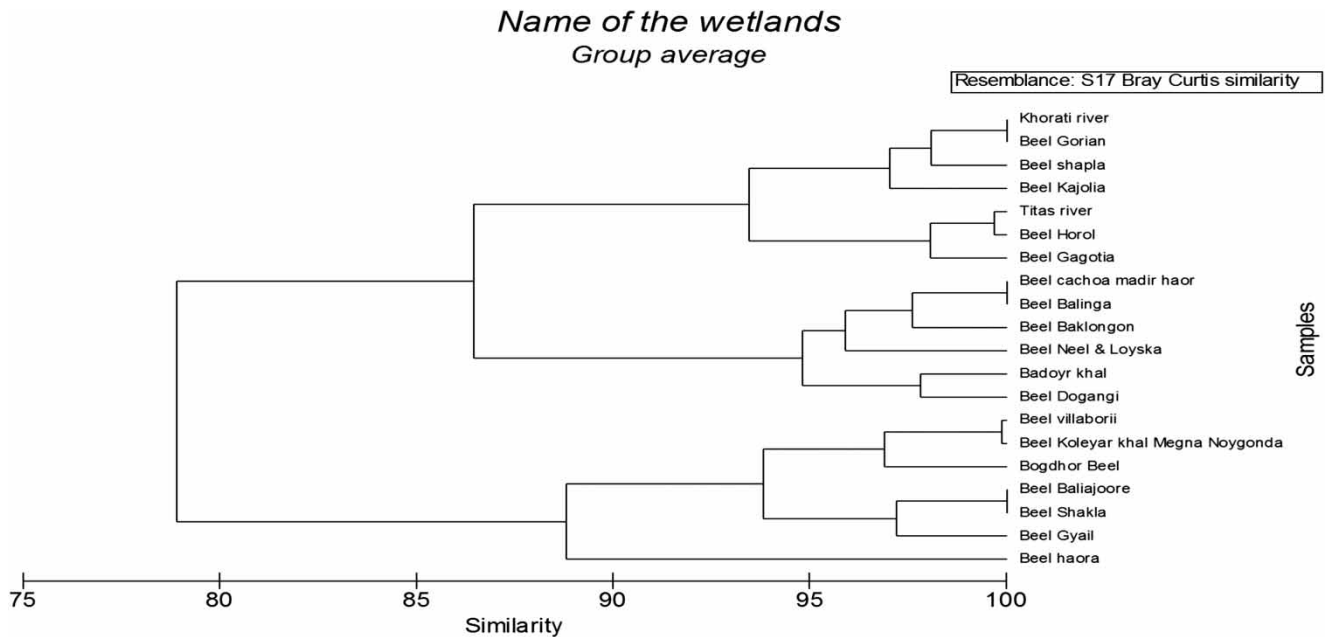
Figure 3 | Dendrogram showing the percentage of similarity among different wetlands of Brahmanbaria district, prepared on the basis of depth.
