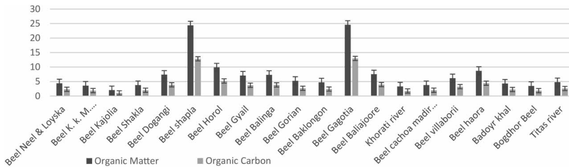
Figure 5 | Percentage of organic matter and organic carbon in different wetlands of Brahmanbaria district.
