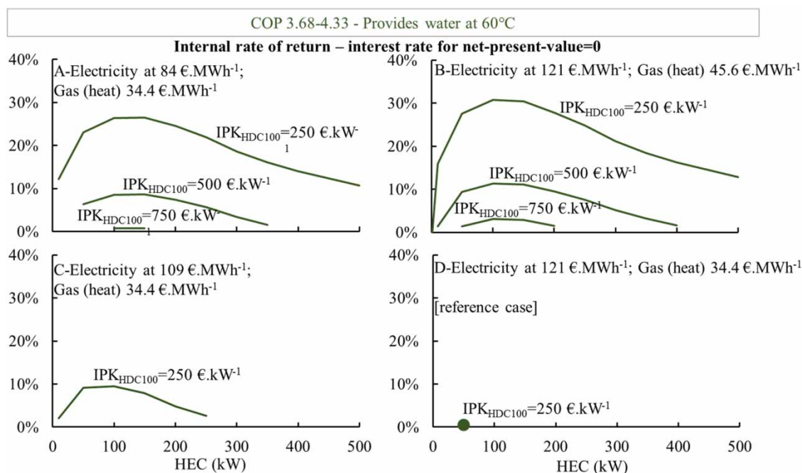
Figure 4 | Electricity and heat prices effects on the internal rate of return (interest rate for a net-present-value = 0). Electricity prices: 121 €·MWh -1 (Euro-area year 2017), 109 €·MWh -1 (2009), 84 €·MWh -1 (production on site); Gas (heat) prices: 34.4 €·MWh -1 (2017), 45.6 €·MWh -1 (2013).
