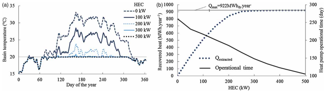
Figure 1 | As functions of the heat extraction capacity (HEC). (a) Basin temperature; (b) Q_{\text{extracted}} : heat extracted and heat pump's operational time.
