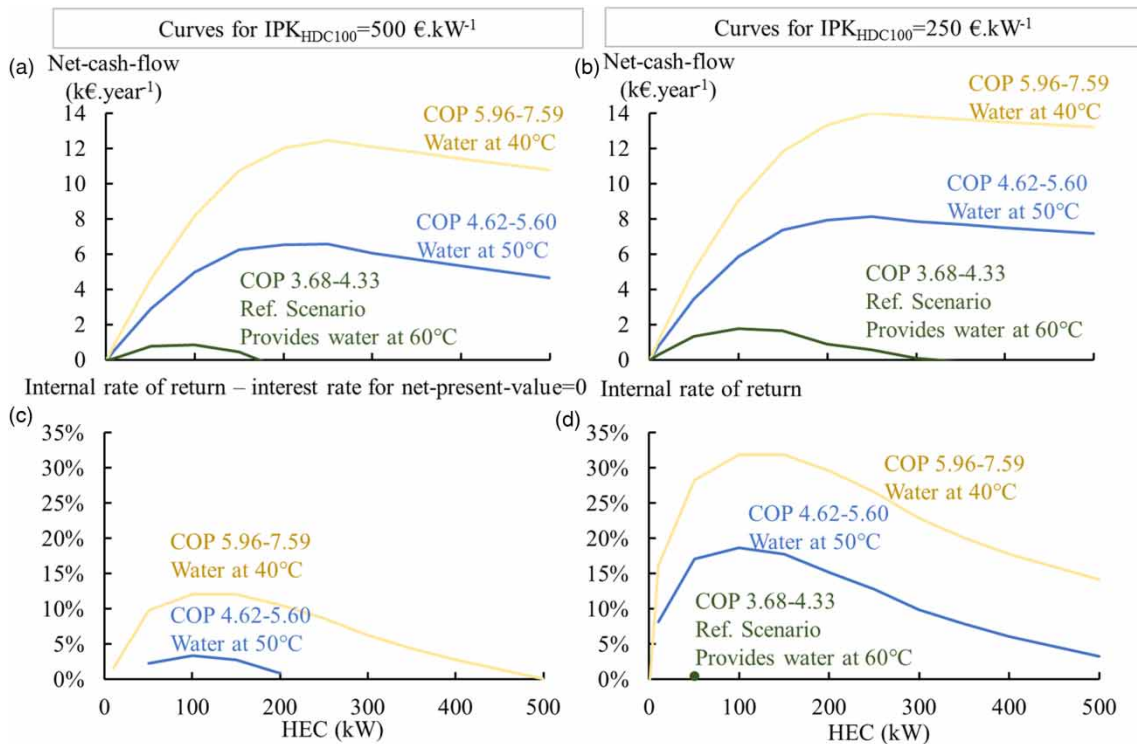
Figure 3 | (Top) Net-cash-flows as a function of the HEC at different COP values. (Bottom) Internal rate of return; this at specific investment costs of IPK_{HDC100} = 500 and 250 \text{ €}\cdot\text{kW}^{-1} [left and right, respectively].
