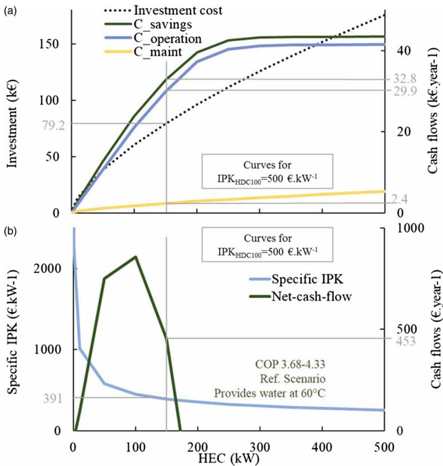
Figure 2 | Economic evaluation at different heat extraction capacities (HEC) considering IPK_{HDC100} = 500 \text{ €}\cdot\text{kW}^{-1} . (a) Savings, operation and maintenance values; (b) investment per kW (IPK) at different HEC, including the effect of scale economics, and the corresponding net-cash-flow. Grey line marks the reference scenario (HEC = 150 kW; see Table 1).
