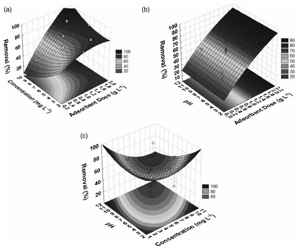
Figure 3 | Response surfaces representing the effects of the interactions between (a) adsorbent dose and concentration, (b) pH and adsorbent dose, (c) pH and concentration.
