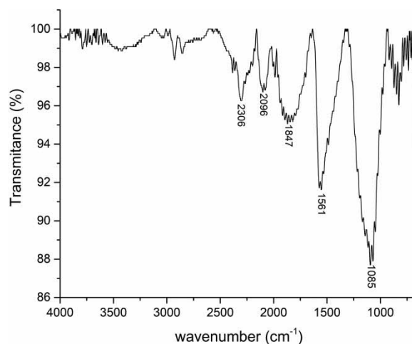
Figure 2 | Fourier transform infrared (FTIR) spectrum of the VAC adsorbent.
