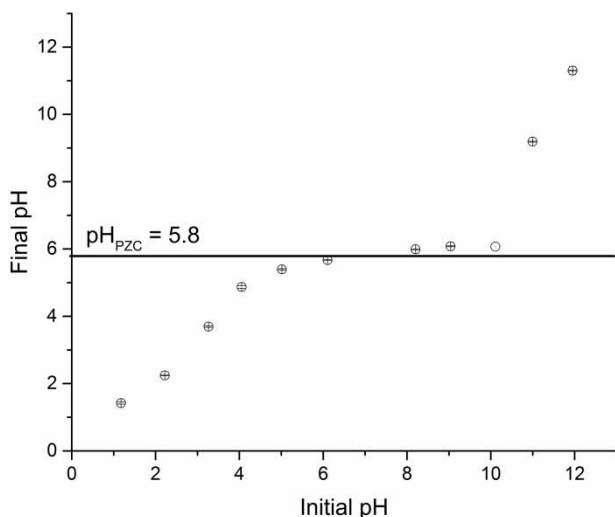
Figure 1 | Experimental data of pH PZC for the adsorbent VAC (160 rpm, 30 °C, adsorbent dose: 1 g/L, contact time: 24 h).
