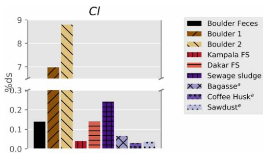
Figure 3 | Occurrence of Cl in fuels, reported as weight percent in fuel dry solids. Sources: a Gold et al. (2017), a Phyllis2.
