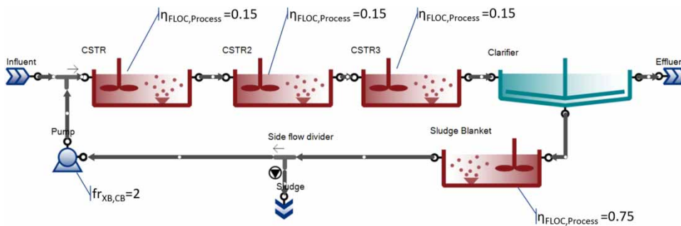
Figure 5 | Rochester (MN) WWTP A-stage configuration and flocculation factors ( \eta_{FLOCC,Process} ) and deflocculation fraction ( f_{r_{xB,CB}} ) applied for each process unit.
