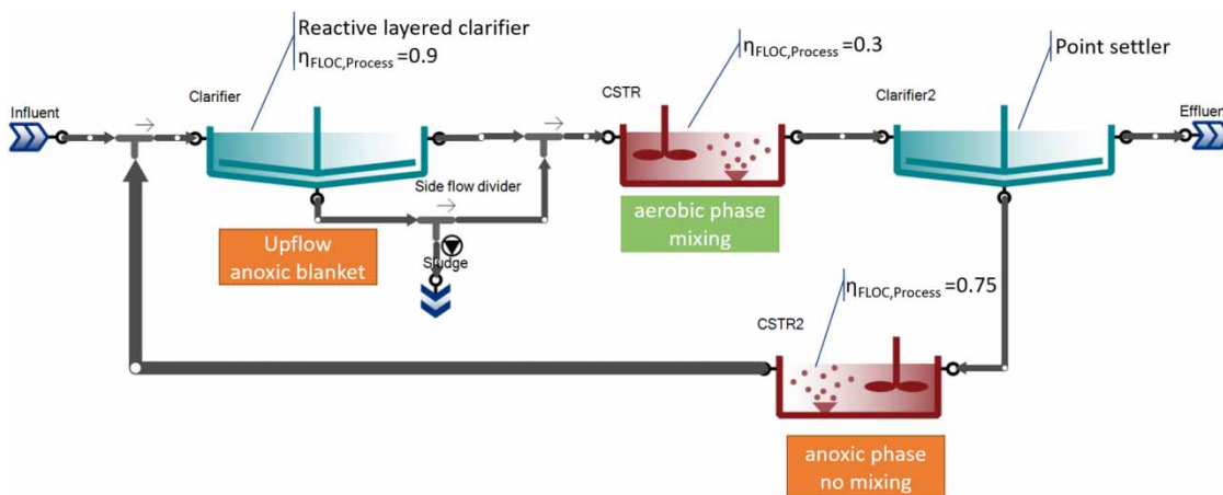
Figure 6 | AAA Rottenburg WWTP A-stage configuration and flocculation factors ( \eta_{FLOCC,Process} ) applied for each process unit.
