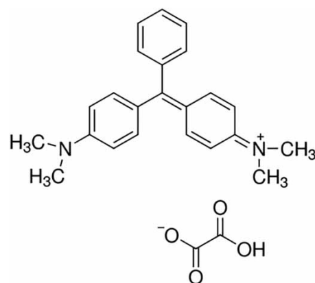
Figure 1 | Molecular structure of MG oxalate.
