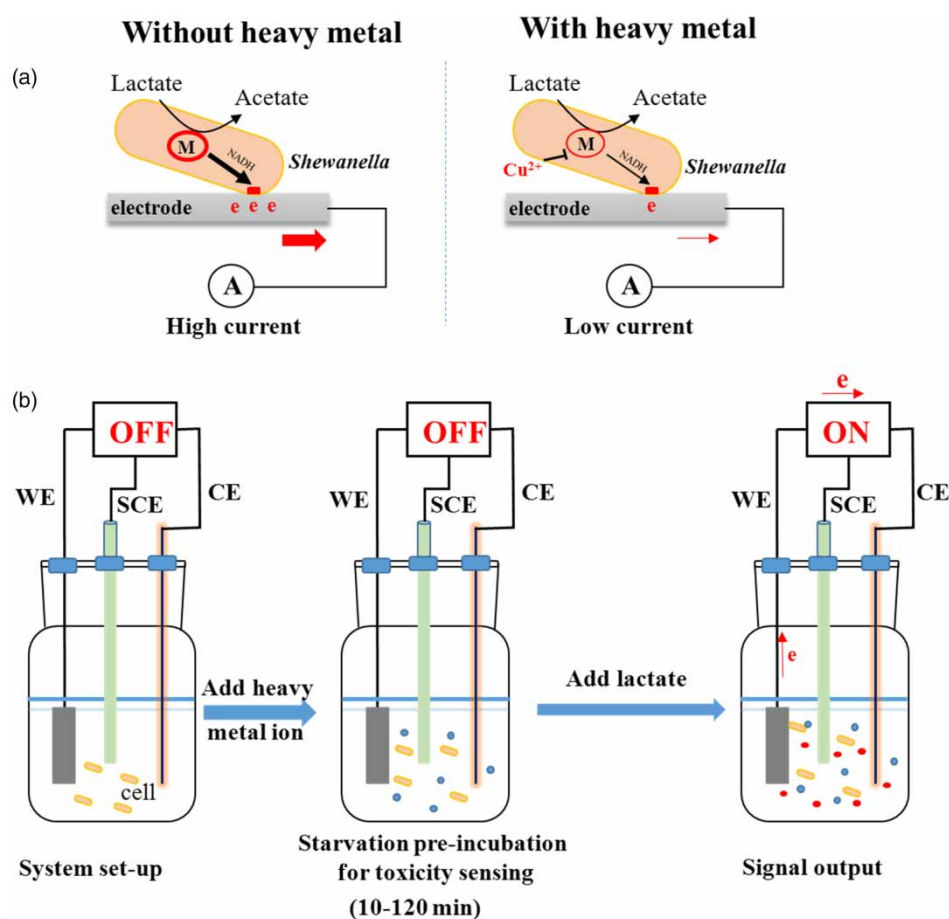
Figure 1 | (a) Schematic of mediator-free Shewanella -based heavy metal toxicity assessment. (b) Operation procedure for starvation pre-incubation integrated heavy metal toxicity biosensing system. Carbon cloth is working electrode (WE), SCE is saturated calomel electrode, and platinum wire is the counter electrode (CE).
