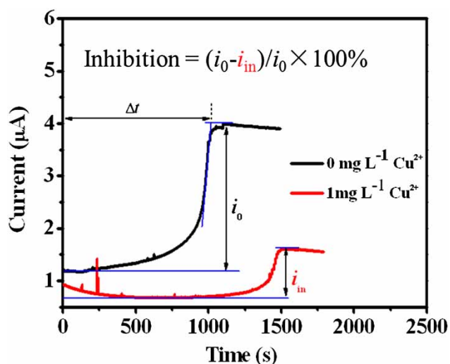
Figure 2 | Amperometric response of Shewanella -based mediator-free biosensor to \text{Cu}^{2+} . The sensing conditions are as follows: starvation pre-incubation with \text{Cu}^{2+} for 30 min, 0.5 V poised potential on WE, and cell density at \text{OD}_{600} = 0.5 .
