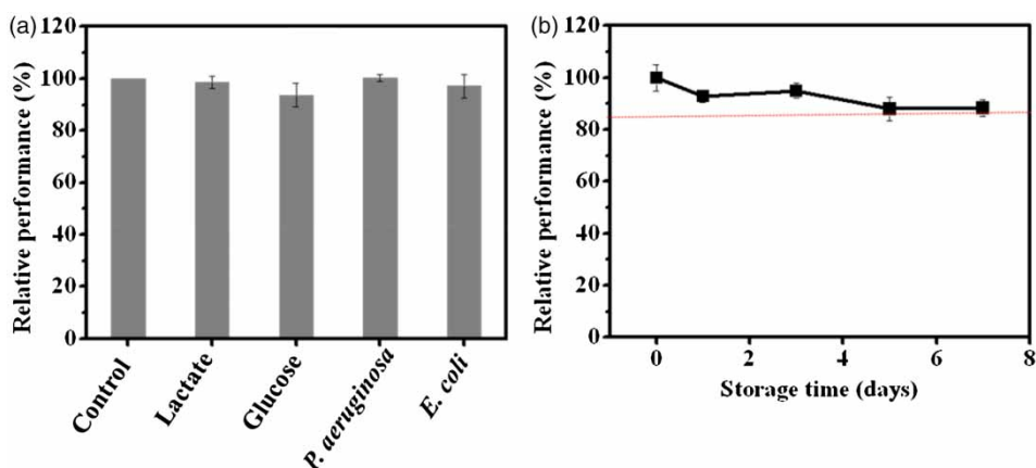
Figure 5 | (a) Interference resistance of the developed biosensor. \text{Cu}^{2+} added is 0.3 \text{ mg L}^{-1} ; The inhibition ratio of \text{Cu}^{2+} without interference (control) was normalized as 100%, while the relative performance was calculated as (inhibition ratio with interference/inhibition ratio of control) \times 100\% . The concentrations of the interferences are as the following: glucose 10 \text{ mM} , lactate 10 \text{ mM} , P. aeruginosa 10^7 \text{ CFU mL}^{-1} , and E. coli 10^7 \text{ CFU mL}^{-1} . Statistical analysis was performed using one-way ANOVA ( P > 0.05 ). (b) Storage stability ( 4^\circ \text{C} ) of the developed biosensor. The inhibition ratio towards 0.3 \text{ mg L}^{-1} \text{ Cu}^{2+} before storage was normalized as 100%.
