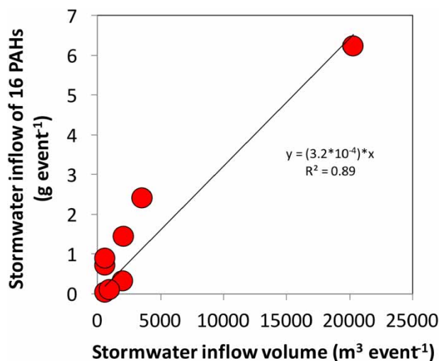
Figure 7 | Relationship between stormwater inflow volume and 16 PAHs.
