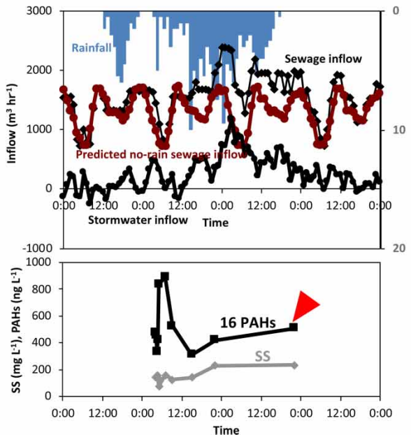
Figure 5 | Sewer inflows during rainfalls (the arrows indicate the samplings that are used for no-rain PAHs concentrations for the rains). (Continued.)
