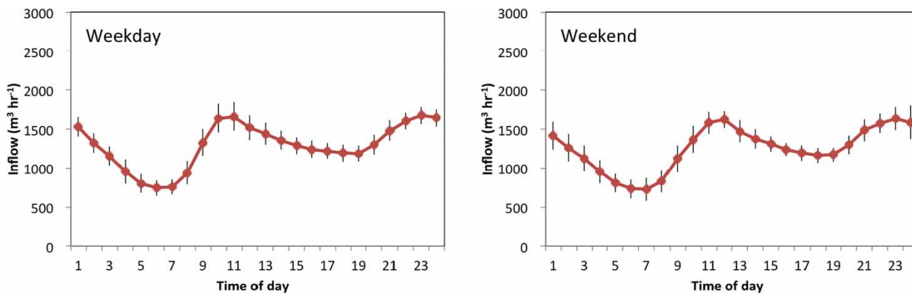
Figure 2 | Yearly mean of sewage inflow volume during no-rainfalls (April 1, 2014–March 31, 2015, total number of days: 181.4 days for weekday and 105.7 days for weekend, \pm bars represent standard deviation).
