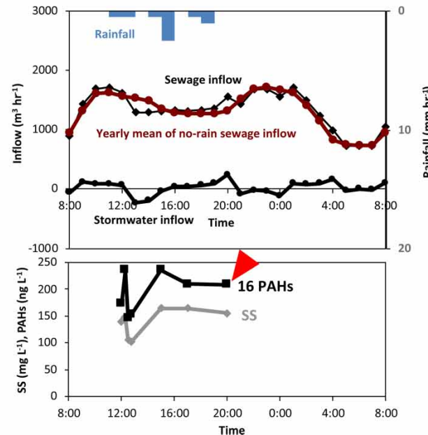
Figure 5 | Sewer inflows during rainfalls (the arrows indicate the samplings that are used for no-rain PAHs concentrations for the rains). (Continued.)
