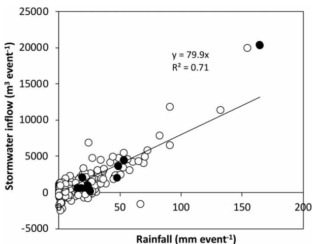
Figure 3 | Relationship between rainfall and stormwater inflow (12/04/01–16/03/31; Filled circles denote the events of PAHs sampling).
