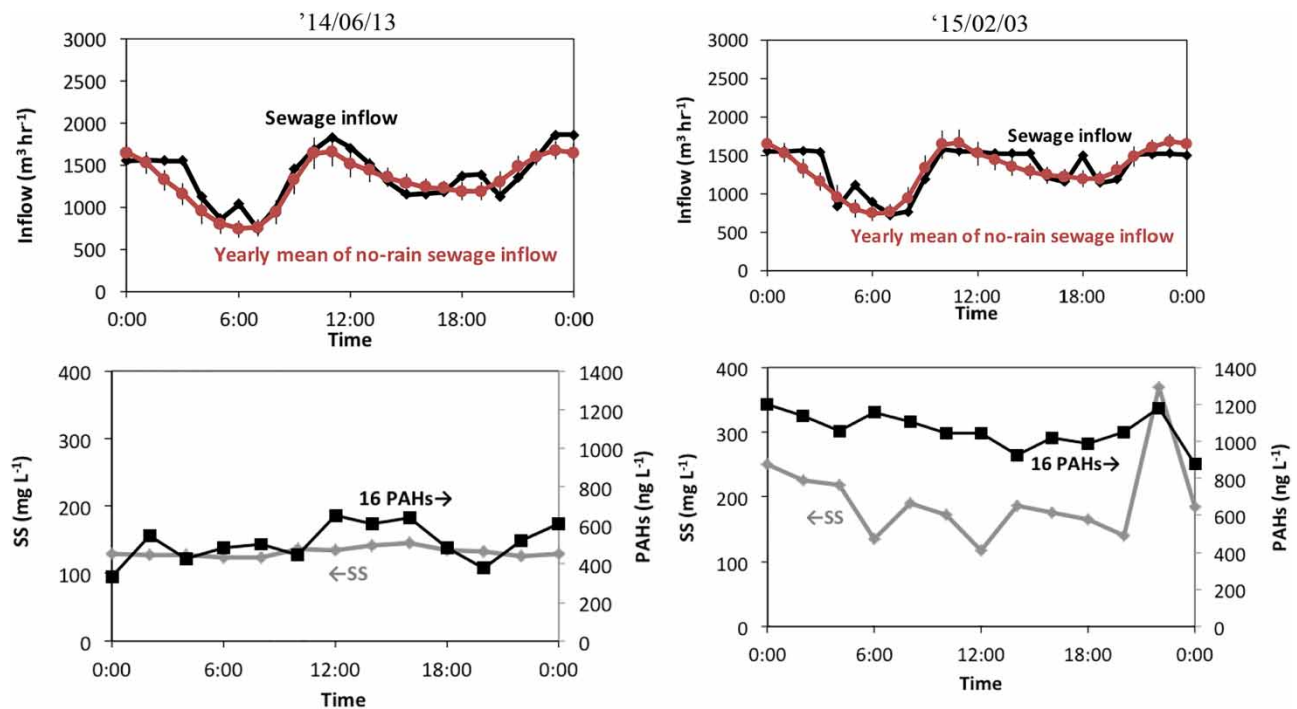
Figure 4 | Diurnal changes of sewage inflow, SS, and 16 PAHs concentrations during no-rain periods.
