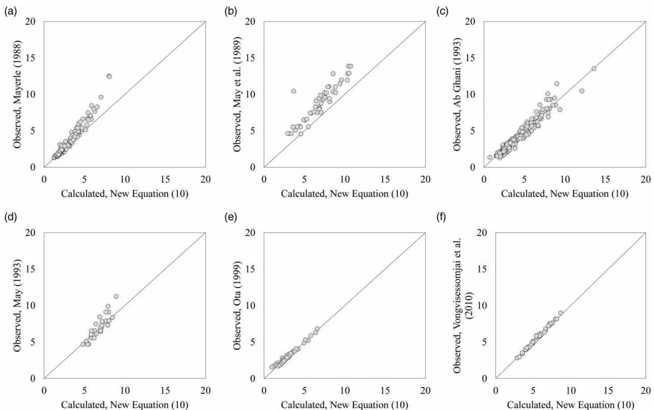
Figure 3 | Comparison of performance of Equation (10) using the experimental data collected in the literature. Data from: (a) Mayerle (1988) ; (b) May et al. (1989) ; (c) Ab Ghani (1993) ; (d) May (1993) ; (e) Ota (1999) ; and (f) Vongvisessomjai et al. (2010) .
