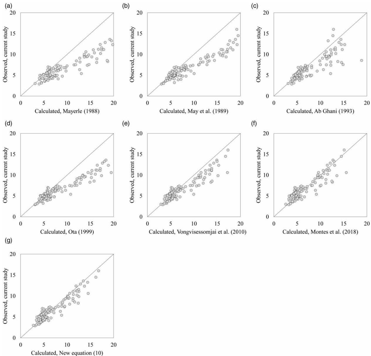
Figure 2 | Comparison of performance of non-deposition without deposited bed models using the experimental data collected for the 595 mm PVC pipe. (a) Mayerle (1988); (b) May et al. (1989); (c) Ab Ghani (1993); (d) Ota (1999); (e) Vongvisessomjai et al. (2010); (f) Montes et al. (2018); and (g) Equation (10).
