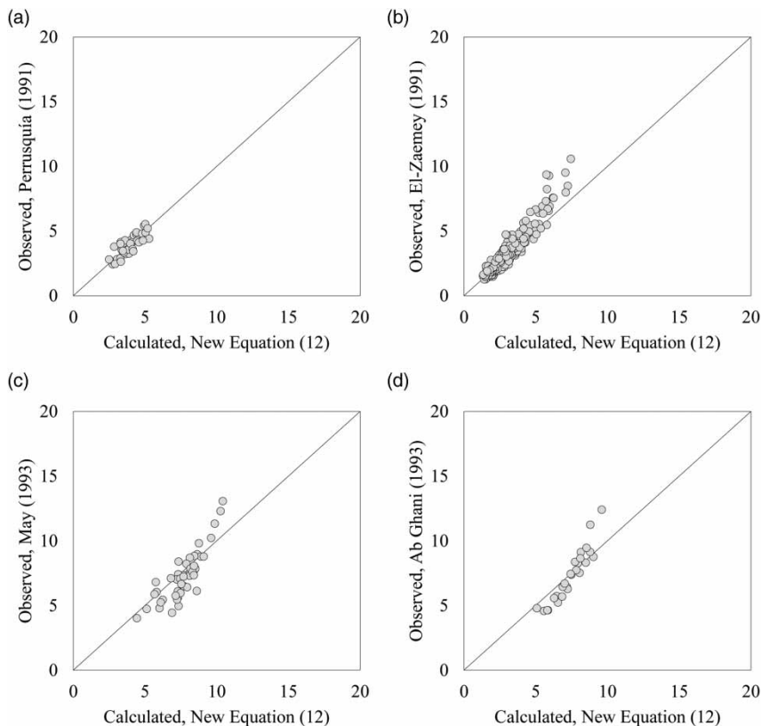
Figure 5 | Comparison of performance of Equation (12) using the experimental data collected from the literature. Data from: (a) Perrusquia (1991); (b) El-Zaemey (1991); (c) May (1993); and (d) Ab Ghani (1993).
