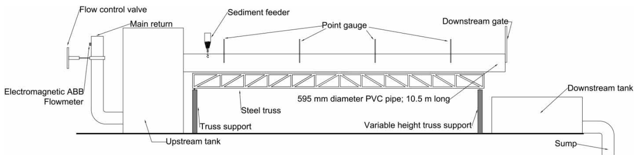
Figure 1 | Schematic diagram of the experimental setup.
