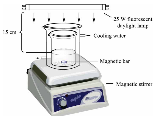
Figure 2 | Reactor of photocatalysis for DBP.
