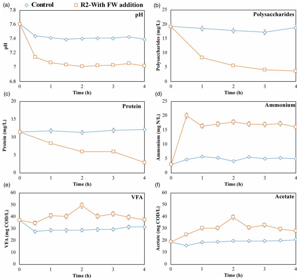
Figure 2 | Hydrolysis of food waste under different conditions. Control: No biofilm attached; R2: Biofilm cultivated with FW addition at sulfate concentration of 40 mg S/L.
