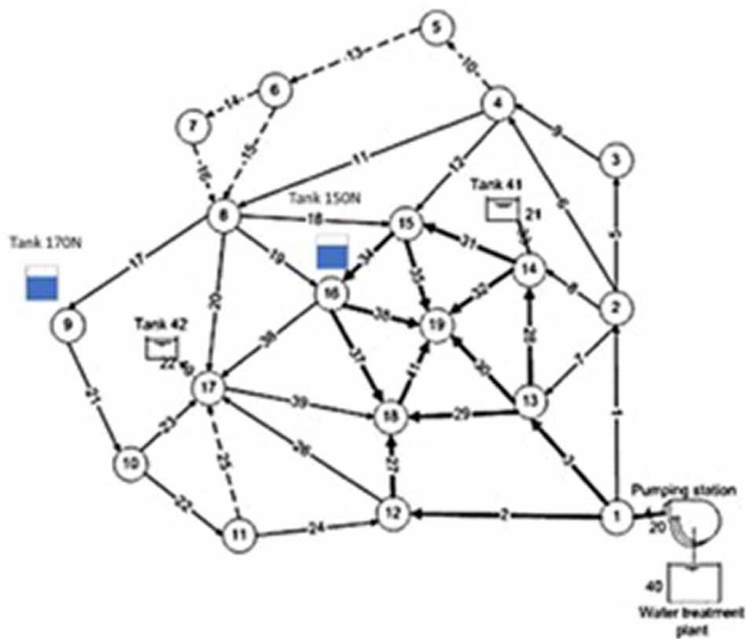
Figure 7 | Vamvakieridou-Lyroudia et al. (2005) and Prasad (2010) solutions. The new tank sizes vary.
