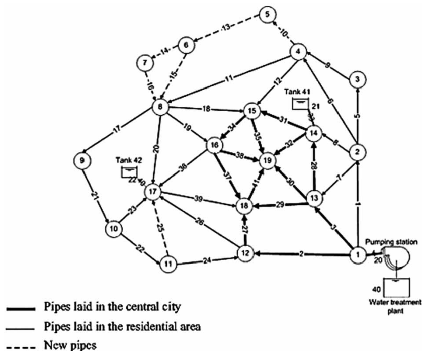
Figure 4 | Anytown Network Problem.
