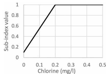
Figure 2 | Chlorine sub-index.
