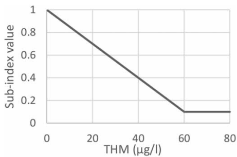
Figure 3 | THM sub-index.
