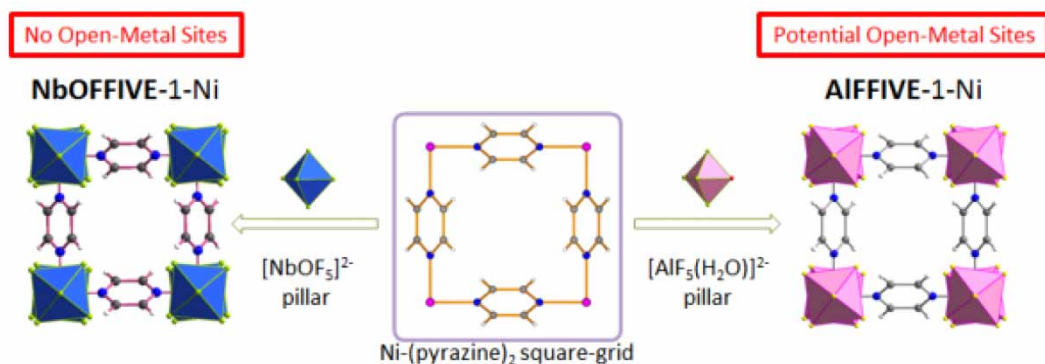
Figure 1 | Schematic showing the subtle difference in the crystal structures of NbOFFIVE-1-Ni and AIFFIVE-1-Ni-1 (Houxiao et al. 2019).
