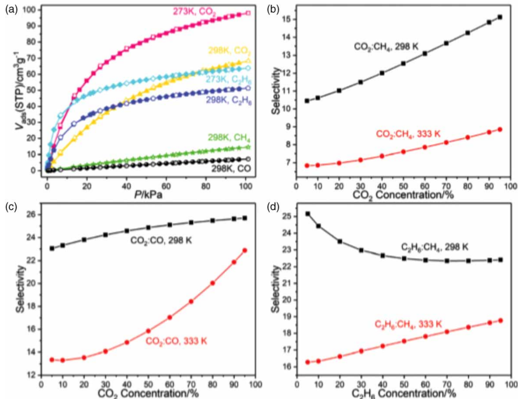
Figure 2 | Gas sorption isotherms of 1a for CO_2 , C_2H_6 , CH_4 and CO at 298 K and CO_2 and C_2H_6 at 273 K (a) and IAST adsorption selectivity of CO_2:CH_4 (b), CO_2:CO (c) and C_2H_6:CH_4 (d) in 1a at 298 and 333 K with a diverse molar mixture (Zhenzhen et al. 2020).
