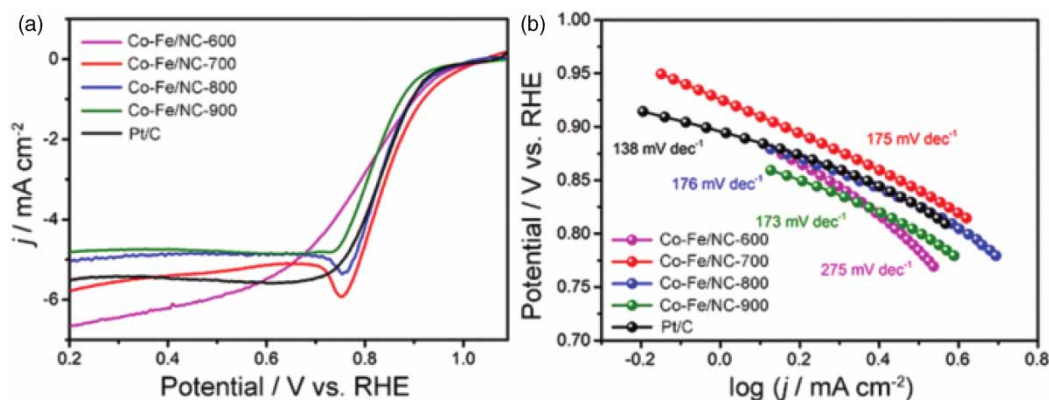
Figure 3 | Electrochemical performance evaluation of Co-Fe/NC composites prepared at different annealing temperatures of 600, 700, 800, and 900 °C. (a) Linear sweep voltammetry (LSV) curves in O 2 -saturated 0.1 M KOH solution with a sweep rate of 10 mV s -1 at the rotating speed of 1,600 rpm. (b) Tafel slope curves (Songlin et al. 2019).
