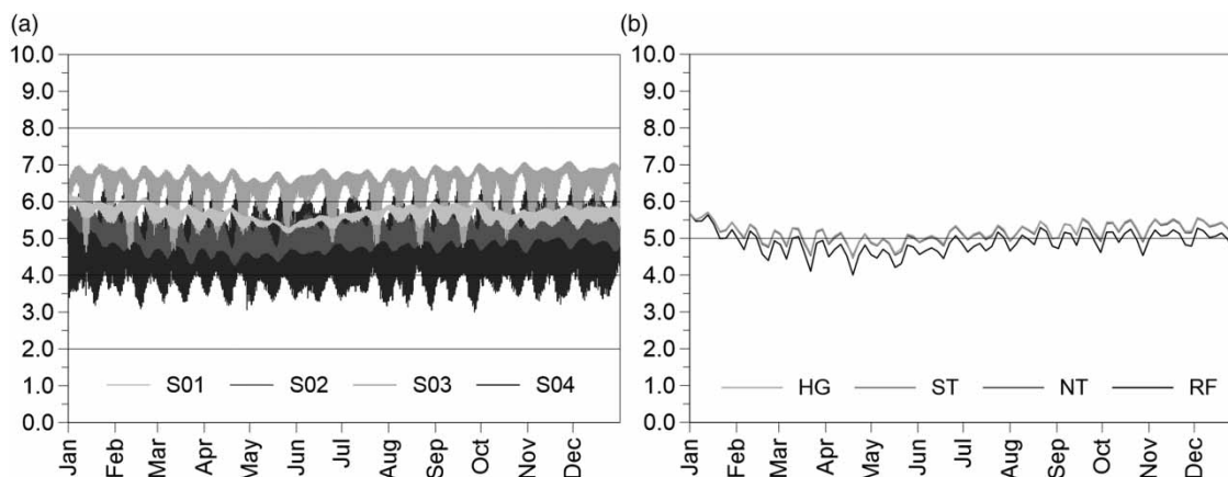
Figure 7 | TRIX index values hourly per station in the HG scenario (a) and daily per scenario at station S02 (b).
