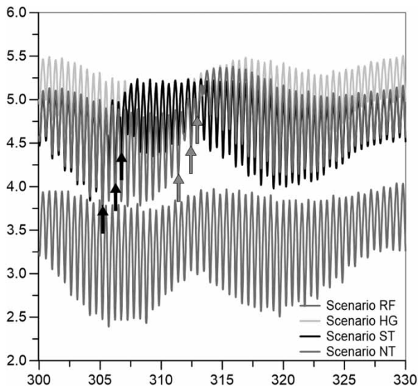
Figure 6 | BOD concentrations at station S01 over a 30-day span in the dry season for different scenarios. Arrows indicate harvests in ST and NT scenarios; time in days.
