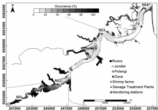
Figure 4 | Map of isolines of current velocities below 0.10 m/s at the end of one-year simulation in the HG scenario.
