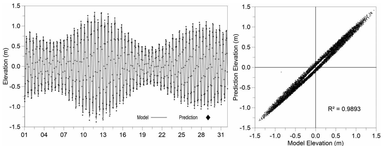
Figure 3 | Forecasted and simulated water level for Natal Harbor.
