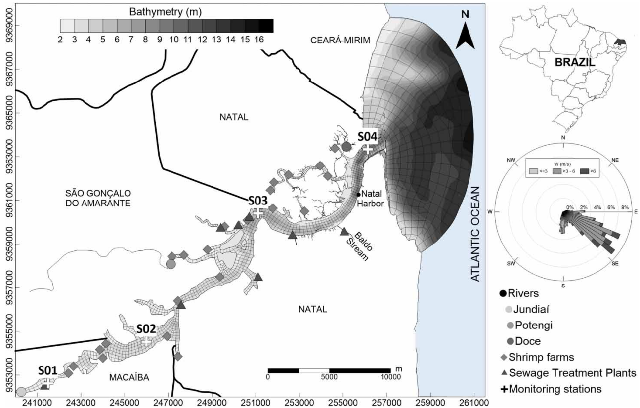
Figure 1 | Modelling domain of PJE with finite element mesh, bathymetry, the position of monitoring stations, tributaries, shrimp farms and sewage effluent plants' discharge points and wind rose representing the time series of the wind from year 2009.
