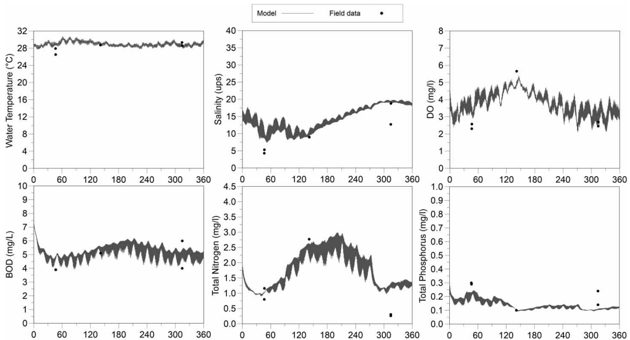
Figure 5 | Model results on S01 for the whole simulation year and field data collected on the station S01. Time in days.
