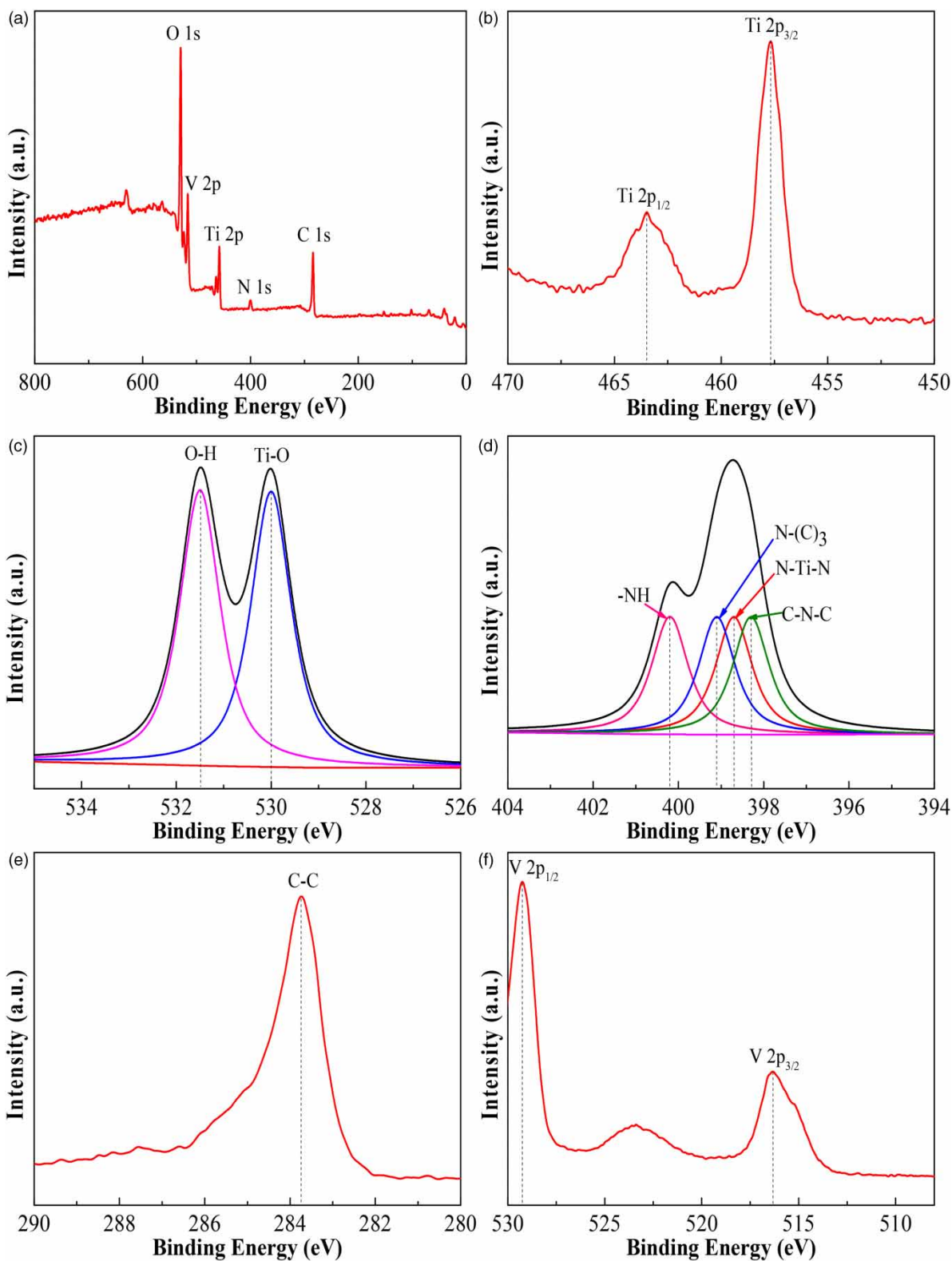
Figure 3 | XPS fully scanned spectra of V/N-TiO 2 -MWCNTs composite (a), XPS spectra of Ti 2p (b), XPS spectra of O 1s (c), XPS spectra of N 1s (d), XPS spectra of C 1s (e) and XPS spectra of V 2p (f).
