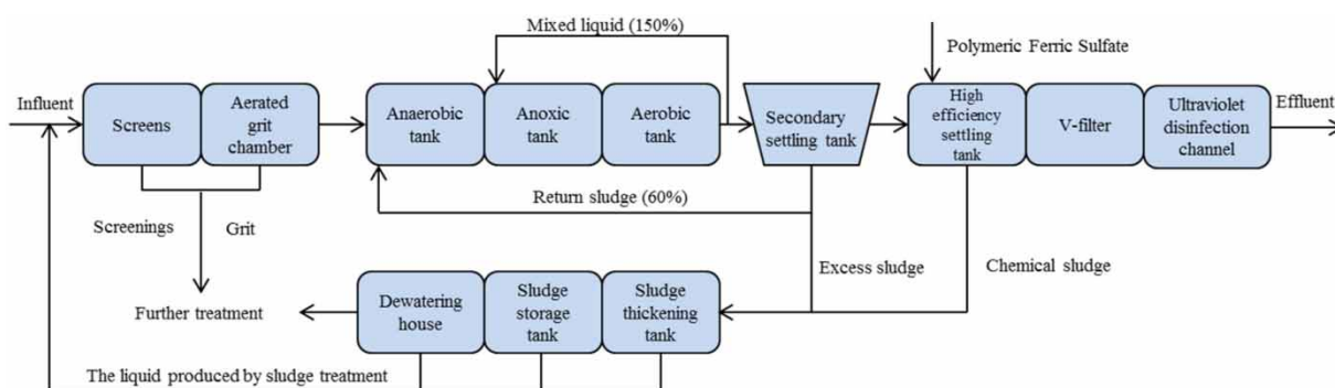
Figure 1 | The flowchart of the sewage treatment plant in Jiangsu Province in China.
