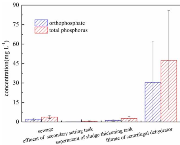
Figure 3 | The concentrations of orthophosphate and total phosphorus at the key sites.
