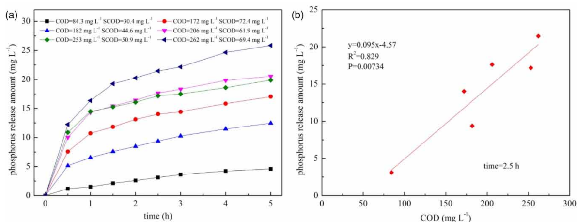
Figure 5 | Phosphorus release with sewage as the general carbon source (a: phosphorus release effect with different COD concentration conditions; b: linear regression of phosphorus release at 2.5 hours).
