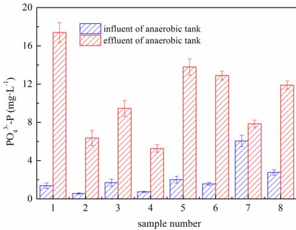
Figure 2 | The changes of orthophosphate concentration in the influent and effluent of the anaerobic tank.
