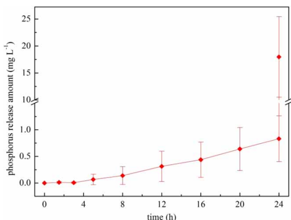
Figure 6 | Phosphorus release with effluent as a lower carbon source.
