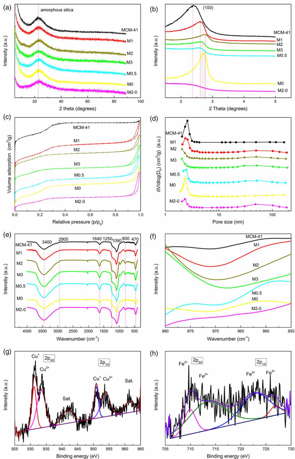
Figure 2 | XRD patterns, nitrogen adsorption isotherms, BJH pore size distributions, FT-IR spectra and XPS spectra of the samples. (a) The large-angle XRD patterns. (b) The small-angle XRD patterns. (c) Nitrogen adsorption isotherms of the samples. (d) BJH pore size distributions of the samples. (e) FT-IR spectra of the samples. (f) Partial FT-IR figure of the samples. (g) XPS spectra of Cu 2p; (h) XPS spectra of Fe 2p.
