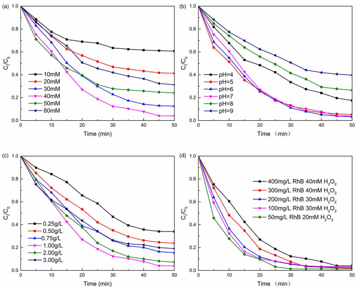
Figure 8 | The effect of the reaction conditions on the RhB degradation. (a) The effect of H_2O_2 dosage on the RhB degradation. (b) The effect of pH on the RhB degradation. (c) The effect of catalyst dosage on the RhB degradation. (d) The effect of dye concentration on the RhB degradation. (Reaction conditions: T = 60^\circ C , pH = 7 , initial dye concentration = 400 mg/L, H_2O_2 dosage = 40 mM and M2 dosage = 1 g/L.)
